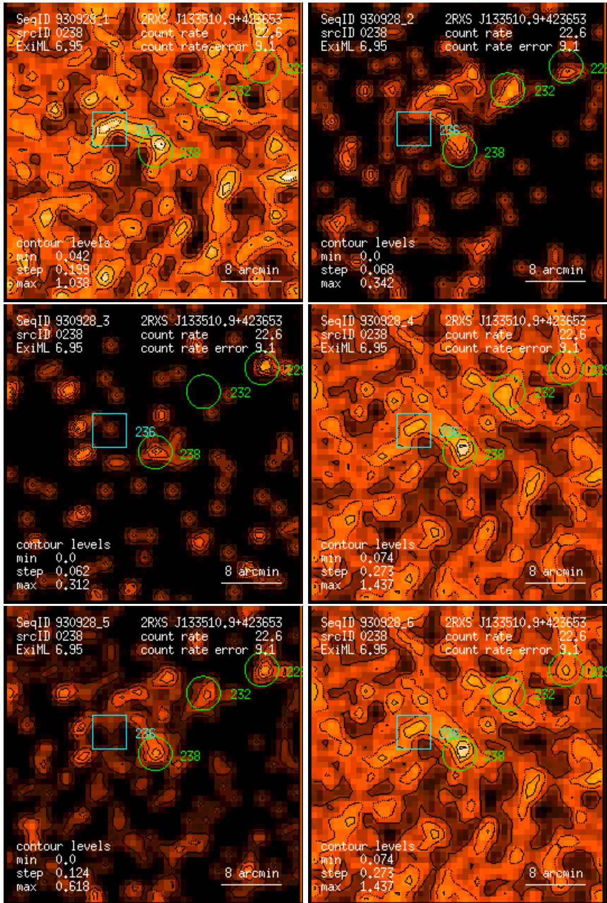
Figure 238: RASS 930928: detection 0238: band rate images, Gaussian filter: (1) PSPC channels 11 – 41, (2) 52 – 90, (3) 91 – 201, (4) 11 – 235, (5) 52 – 201, (6) 11 – 201. Broad band rates in counts/ks. Band rate contour levels in counts/ks/arcmin 2 .
