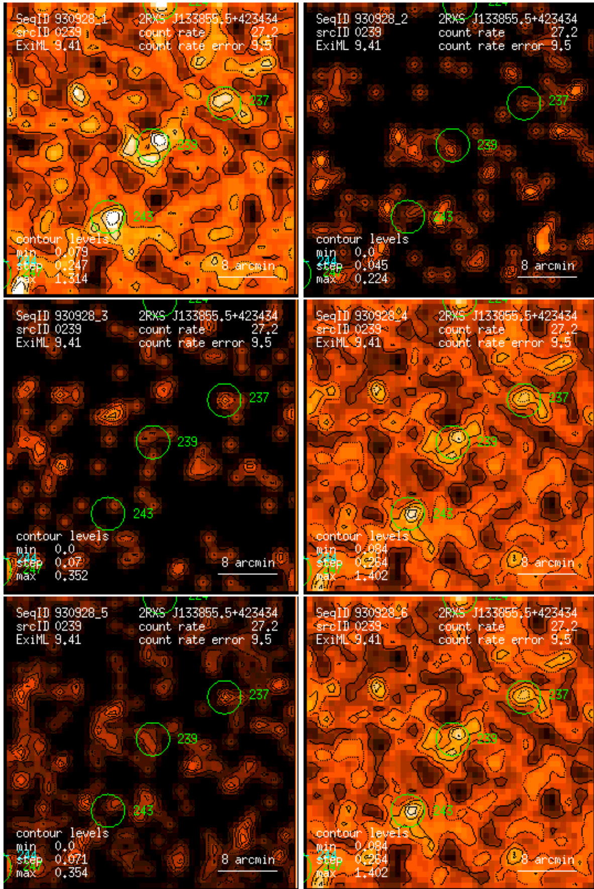
Figure 239: RASS 930928: detection 0239: band rate images, Gaussian filter: (1) PSPC channels 11 – 41, (2) 52 – 90, (3) 91 – 201, (4) 11 – 235, (5) 52 – 201, (6) 11 – 201. Broad band rates in counts/ks. Band rate contour levels in counts/ks/arcmin 2 .
