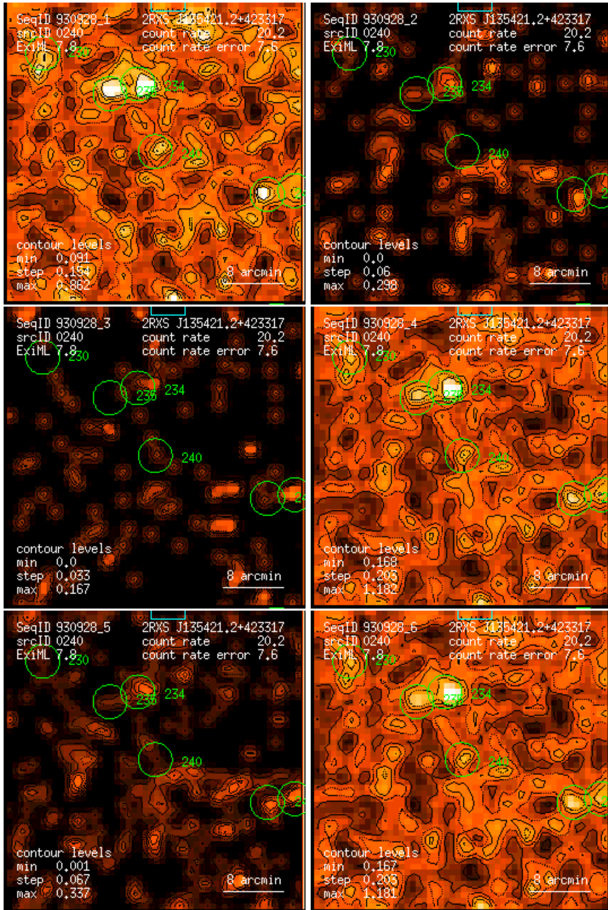
Figure 240: RASS 930928: detection 0240: band rate images, Gaussian filter: (1) PSPC channels 11 – 41, (2) 52 – 90, (3) 91 – 201, (4) 11 – 235, (5) 52 – 201, (6) 11 – 201. Broad band rates in counts/ks. Band rate contour levels in counts/ks/arcmin 2 .
