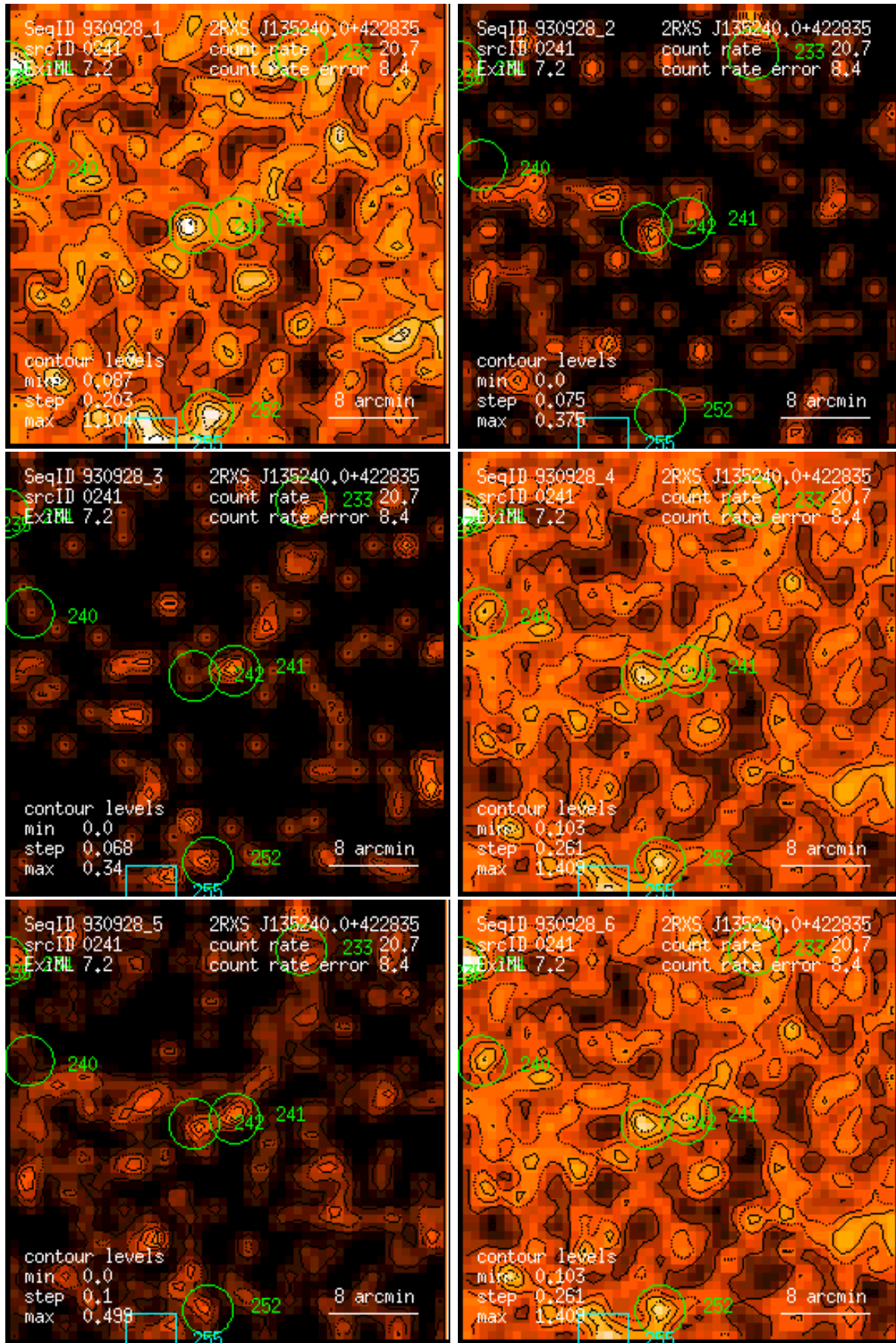
Figure 241: RASS 930928: detection 0241: band rate images, Gaussian filter: (1) PSPC channels 11 – 41, (2) 52 – 90, (3) 91 – 201, (4) 11 – 235, (5) 52 – 201, (6) 11 – 201. Broad band rates in counts/ks. Band rate contour levels in counts/ks/arcmin 2 .
