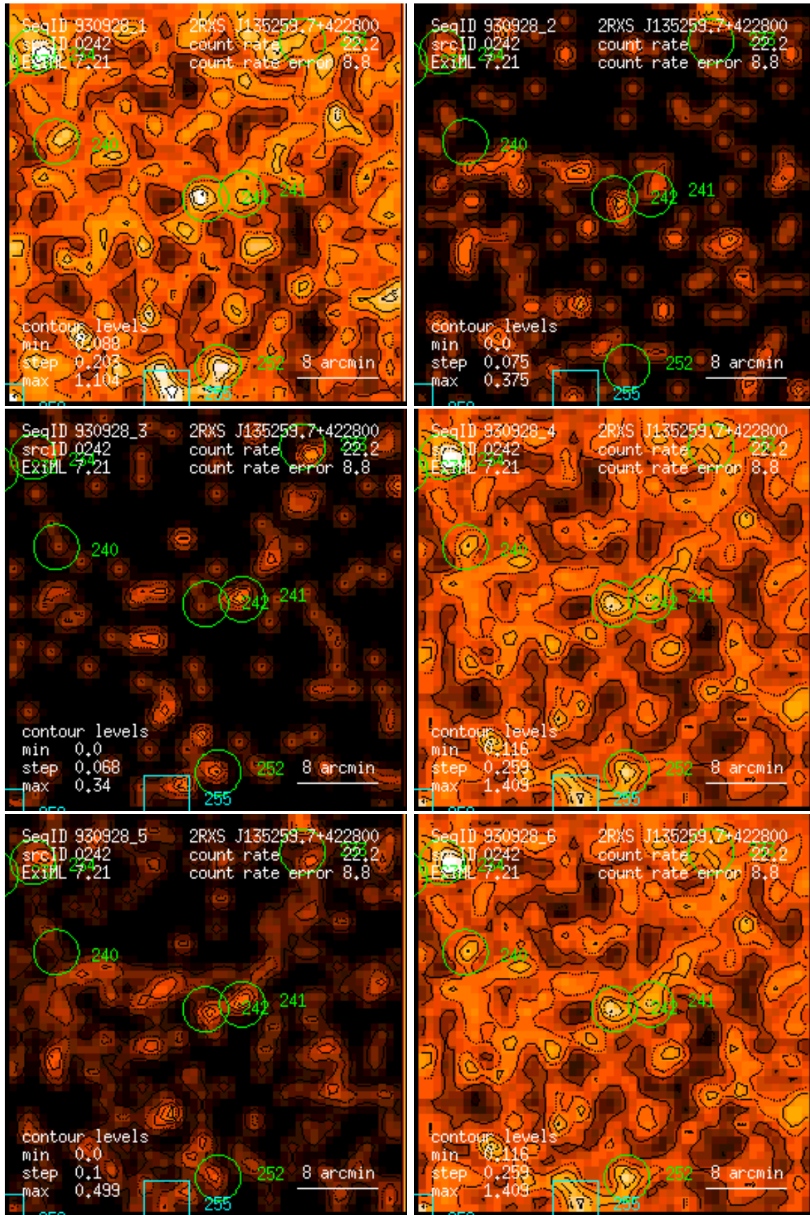
Figure 242: RASS 930928: detection 0242: band rate images, Gaussian filter: (1) PSPC channels 11 – 41, (2) 52 – 90, (3) 91 – 201, (4) 11 – 235, (5) 52 – 201, (6) 11 – 201. Broad band rates in counts/ks. Band rate contour levels in counts/ks/arcmin 2 .
