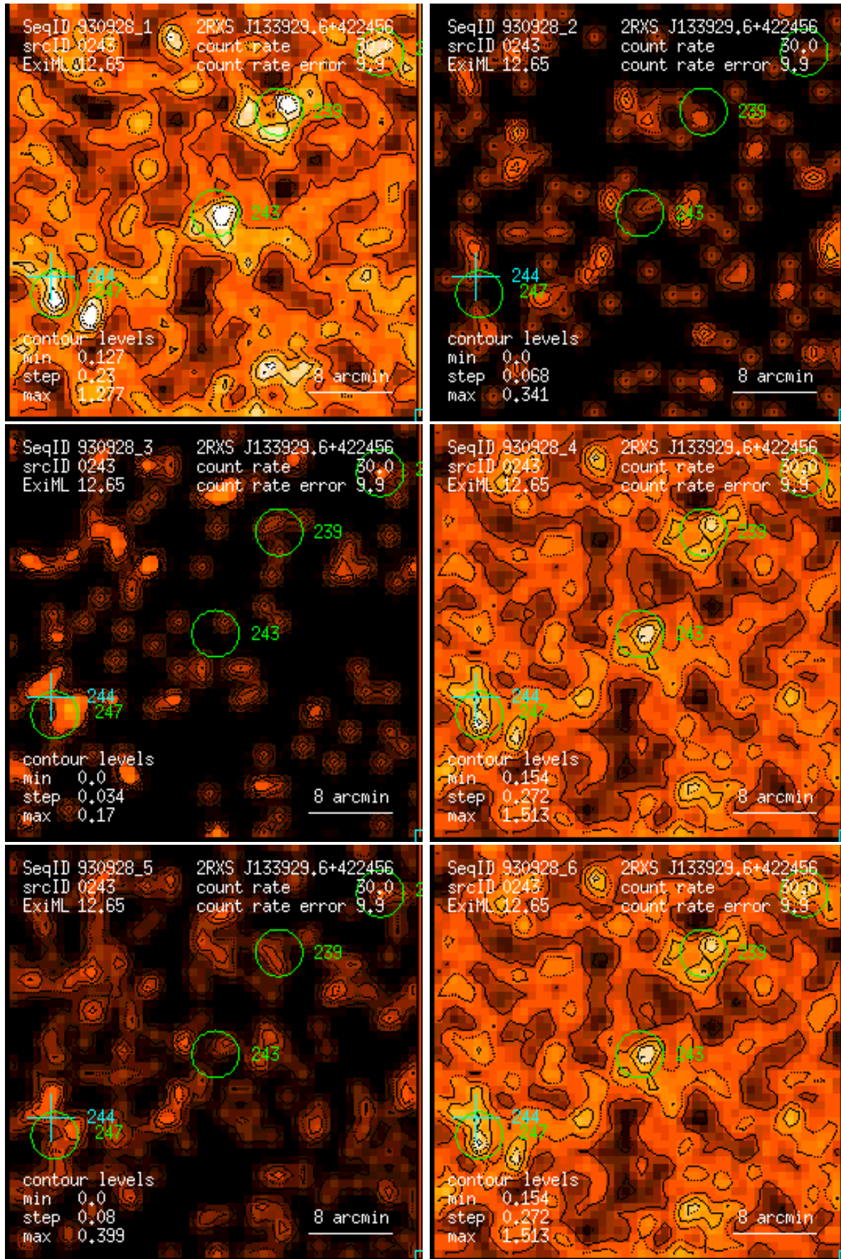
Figure 243: RASS 930928: detection 0243: band rate images, Gaussian filter: (1) PSPC channels 11 – 41, (2) 52 – 90, (3) 91 – 201, (4) 11 – 235, (5) 52 – 201, (6) 11 – 201. Broad band rates in counts/ks. Band rate contour levels in counts/ks/arcmin 2 .
