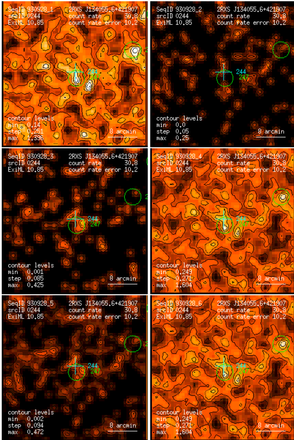
Figure 244: RASS 930928: detection 0244: band rate images, Gaussian filter: (1) PSPC channels 11 – 41, (2) 52 – 90, (3) 91 – 201, (4) 11 – 235, (5) 52 – 201, (6) 11 – 201. Broad band rates in counts/ks. Band rate contour levels in counts/ks/arcmin 2 .
