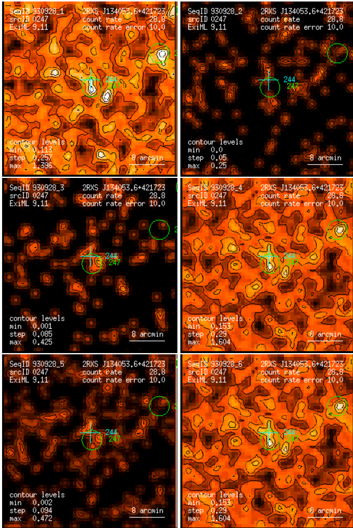
Figure 247: RASS 930928: detection 0247: band rate images, Gaussian filter: (1) PSPC channels 11 – 41, (2) 52 – 90, (3) 91 – 201, (4) 11 – 235, (5) 52 – 201, (6) 11 – 201. Broad band rates in counts/ks. Band rate contour levels in counts/ks/arcmin 2 .
