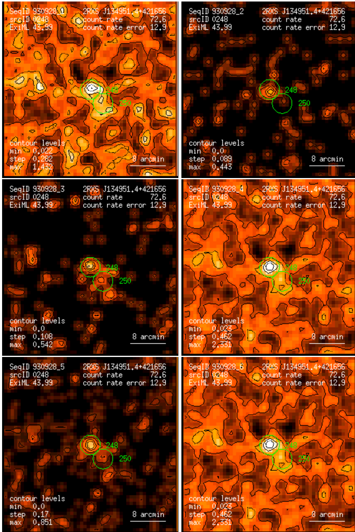
Figure 248: RASS 930928: detection 0248: band rate images, Gaussian filter: (1) PSPC channels 11 – 41, (2) 52 – 90, (3) 91 – 201, (4) 11 – 235, (5) 52 – 201, (6) 11 – 201. Broad band rates in counts/ks. Band rate contour levels in counts/ks/arcmin 2 .
