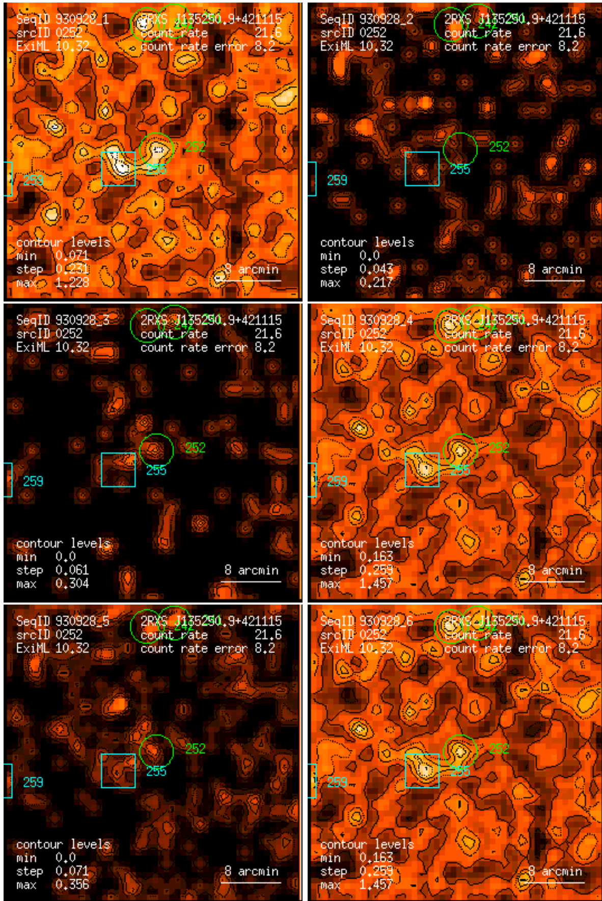
Figure 252: RASS 930928: detection 0252: band rate images, Gaussian filter: (1) PSPC channels 11 – 41, (2) 52 – 90, (3) 91 – 201, (4) 11 – 235, (5) 52 – 201, (6) 11 – 201. Broad band rates in counts/ks. Band rate contour levels in counts/ks/arcmin 2 .
