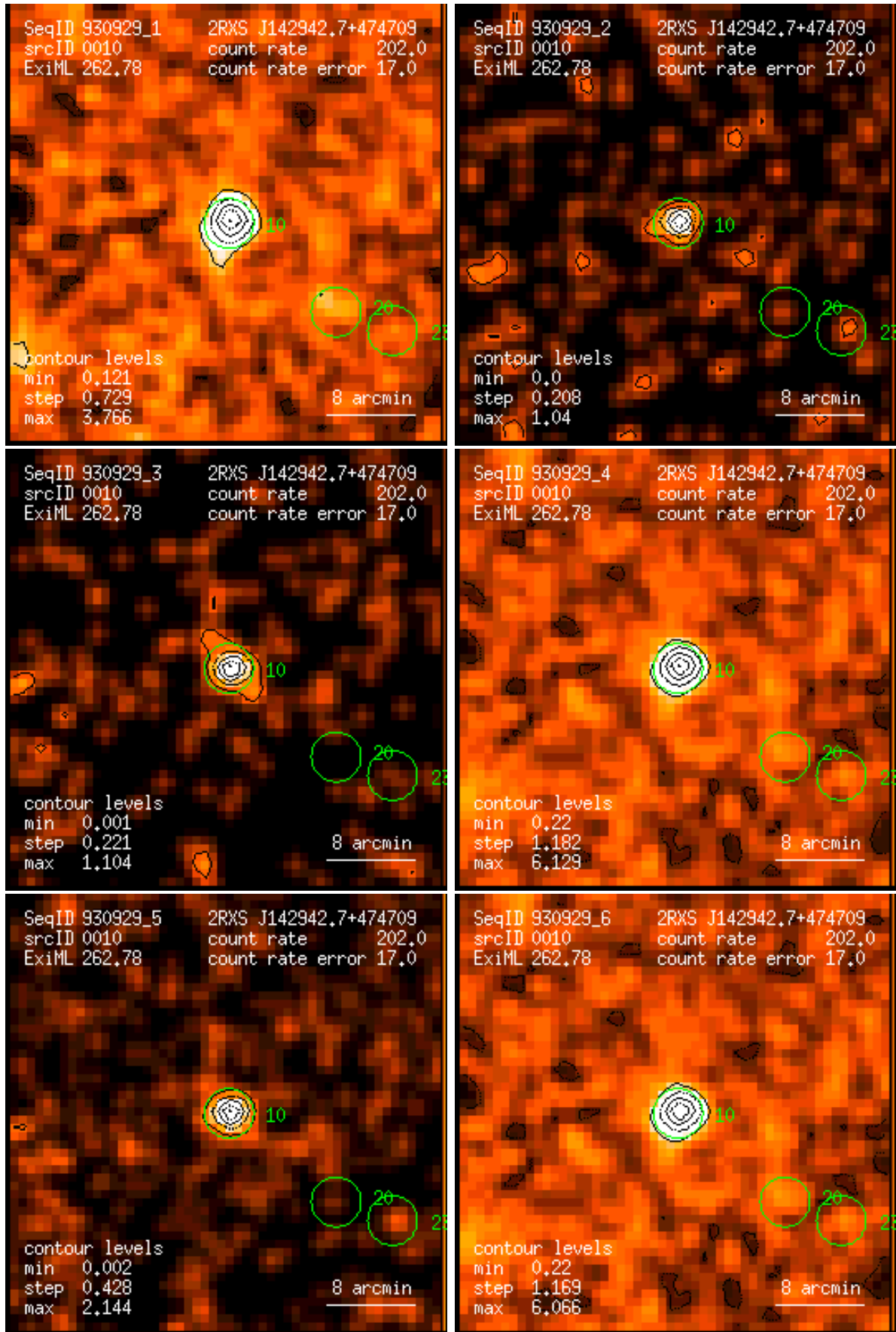
Figure 10: RASS 930929: detection 0010: band rate images, Gaussian filter: (1) PSPC channels 11 – 41, (2) 52 – 90, (3) 91 – 201, (4) 11 – 235, (5) 52 – 201, (6) 11 – 201. Broad band rates in counts/ks. Band rate contour levels in counts/ks/arcmin 2 .
