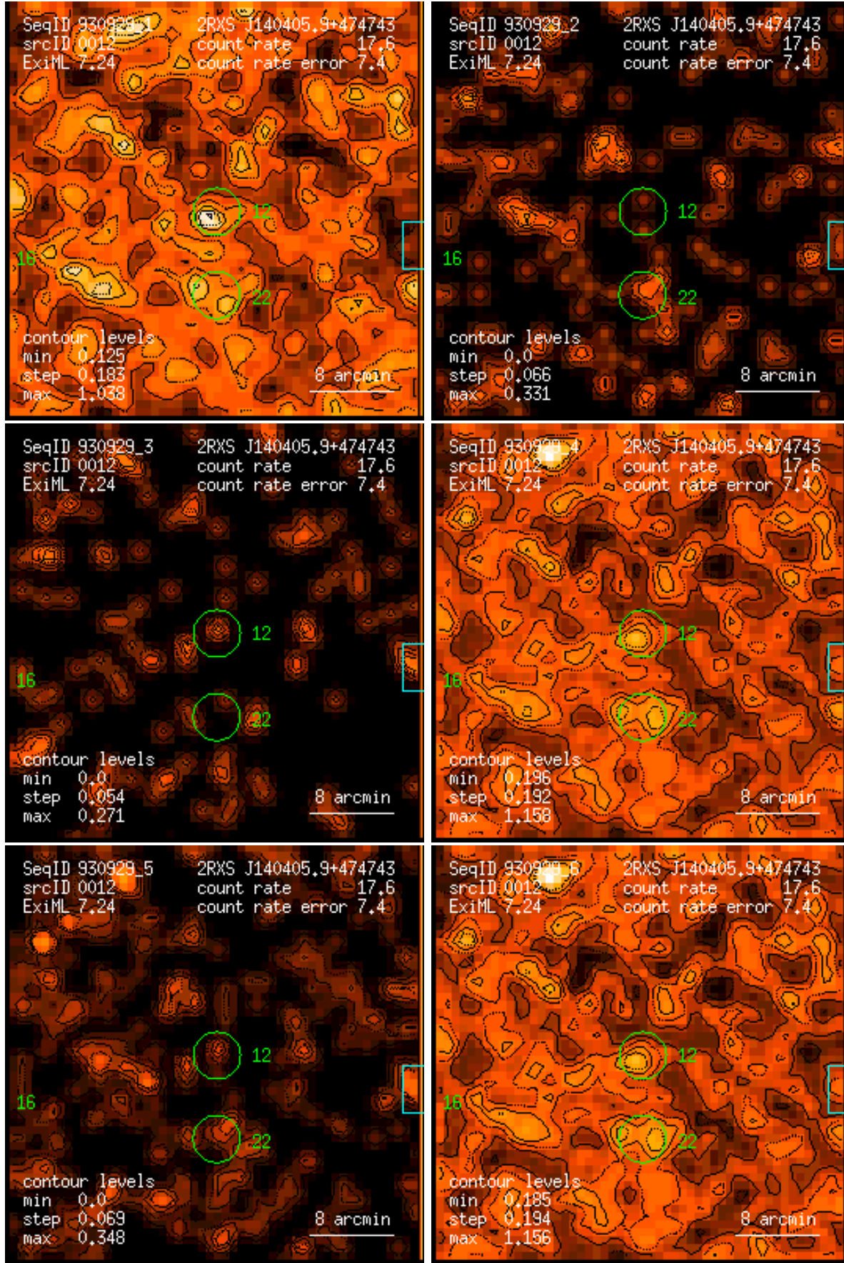
Figure 12: RASS 930929: detection 0012: band rate images, Gaussian filter: (1) PSPC channels 11 – 41, (2) 52 – 90, (3) 91 – 201, (4) 11 – 235, (5) 52 – 201, (6) 11 – 201. Broad band rates in counts/ks. Band rate contour levels in counts/ks/arcmin 2 .
