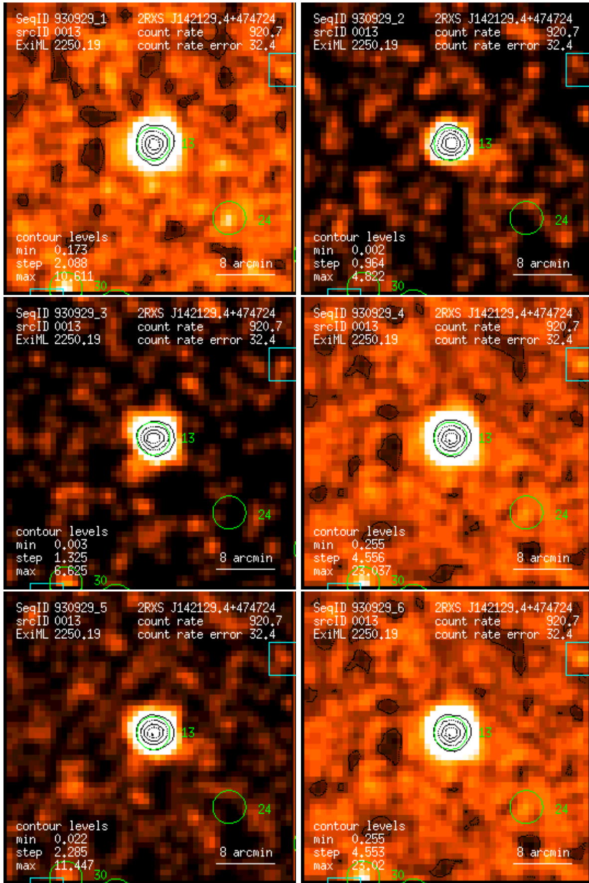
Figure 13: RASS 930929: detection 0013: band rate images, Gaussian filter: (1) PSPC channels 11 – 41, (2) 52 – 90, (3) 91 – 201, (4) 11 – 235, (5) 52 – 201, (6) 11 – 201. Broad band rates in counts/ks. Band rate contour levels in counts/ks/arcmin 2 .
