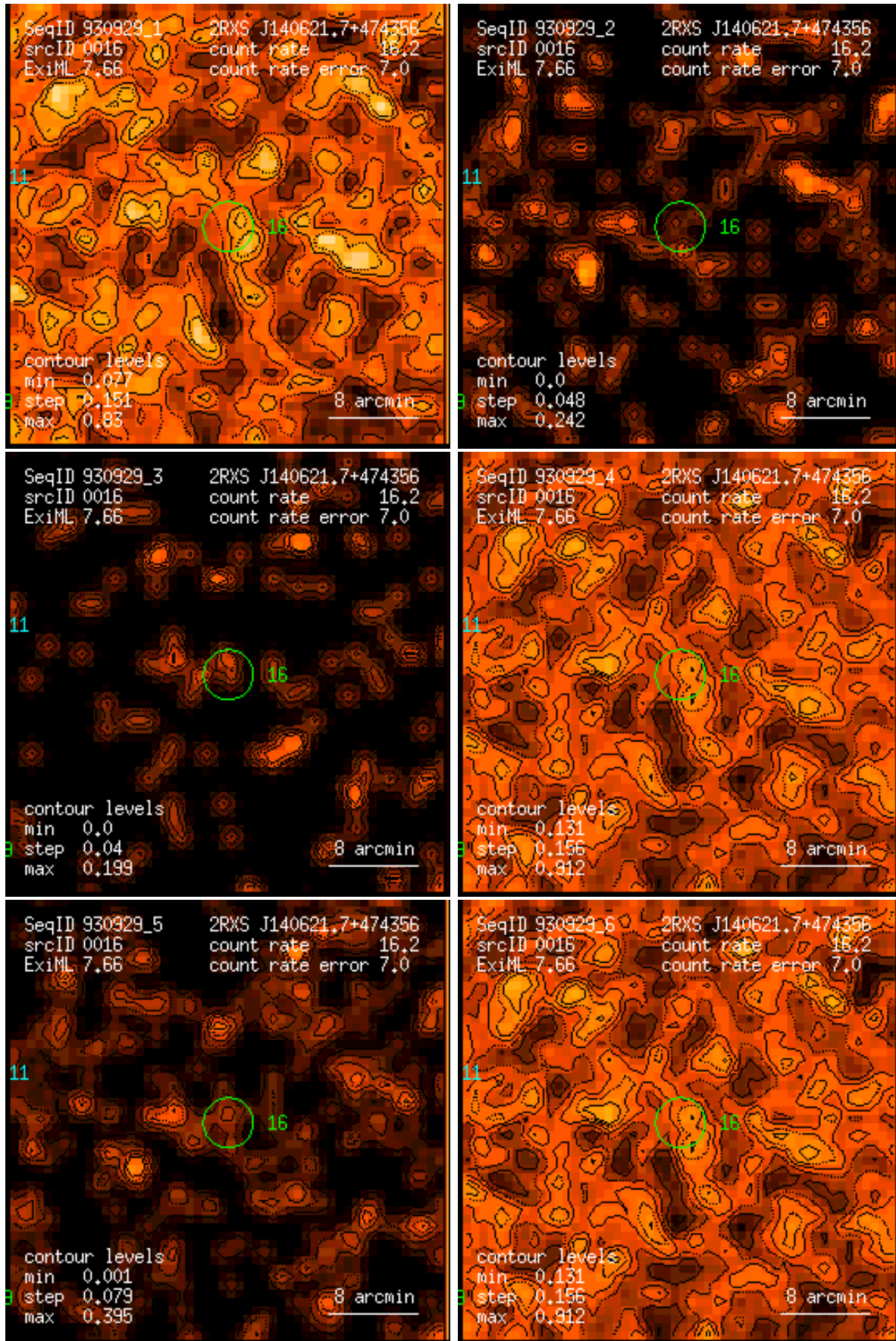
Figure 16: RASS 930929: detection 0016: band rate images, Gaussian filter: (1) PSPC channels 11 – 41, (2) 52 – 90, (3) 91 – 201, (4) 11 – 235, (5) 52 – 201, (6) 11 – 201. Broad band rates in counts/ks. Band rate contour levels in counts/ks/arcmin 2 .
