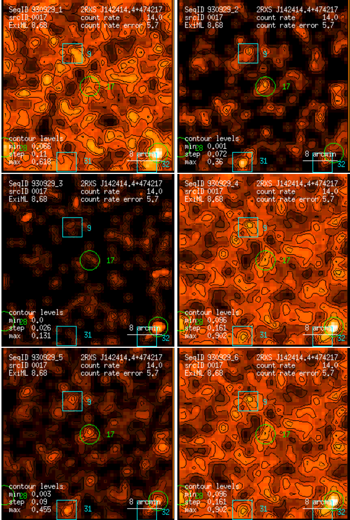
Figure 17: RASS 930929: detection 0017: band rate images, Gaussian filter: (1) PSPC channels 11 – 41, (2) 52 – 90, (3) 91 – 201, (4) 11 – 235, (5) 52 – 201, (6) 11 – 201. Broad band rates in counts/ks. Band rate contour levels in counts/ks/arcmin 2 .
