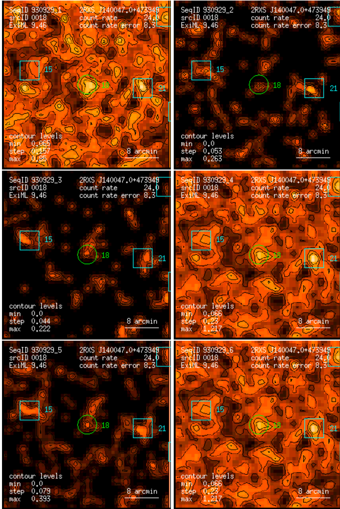
Figure 18: RASS 930929: detection 0018: band rate images, Gaussian filter: (1) PSPC channels 11 – 41, (2) 52 – 90, (3) 91 – 201, (4) 11 – 235, (5) 52 – 201, (6) 11 – 201. Broad band rates in counts/ks. Band rate contour levels in counts/ks/arcmin 2 .
