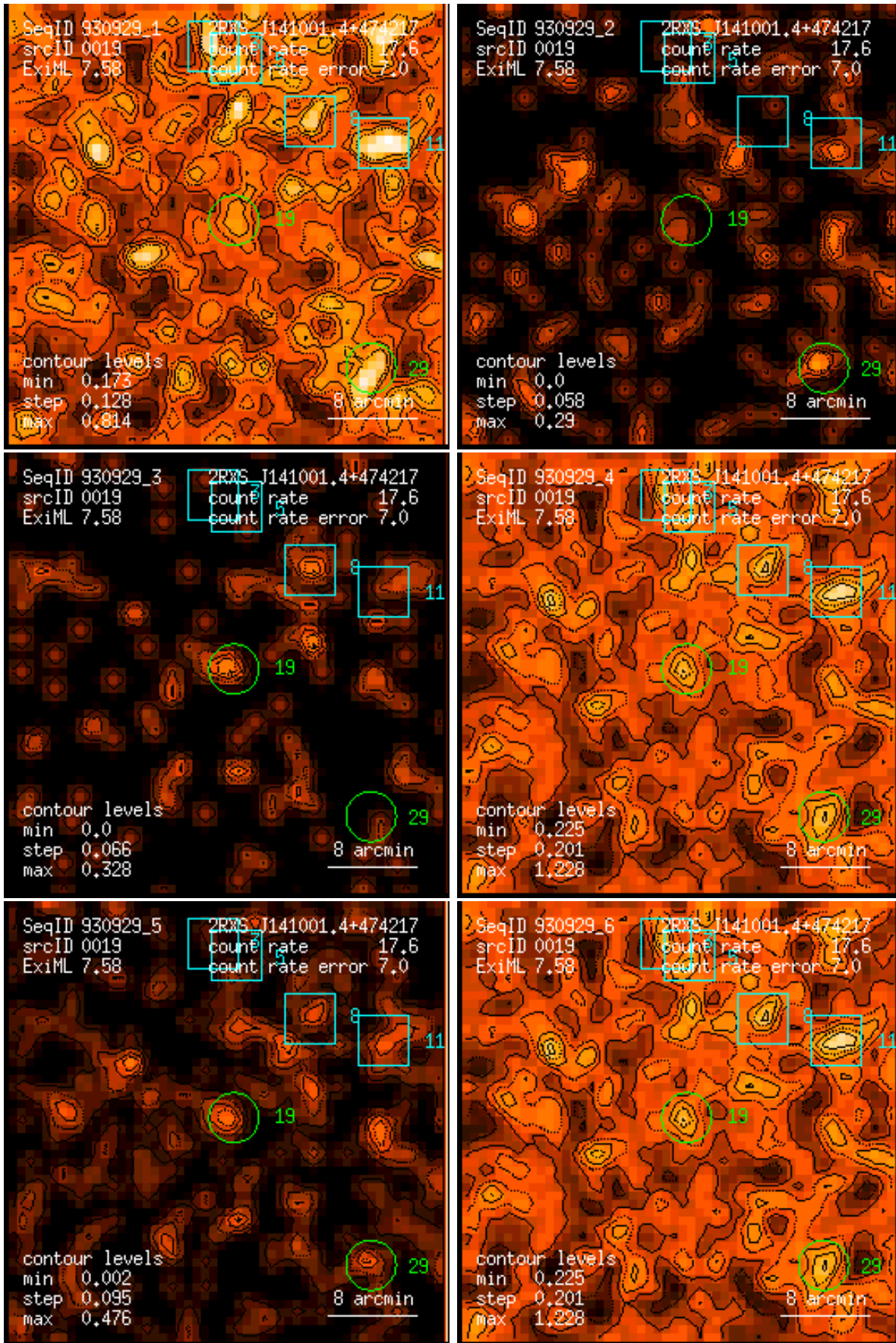
Figure 19: RASS 930929: detection 0019: band rate images, Gaussian filter: (1) PSPC channels 11 – 41, (2) 52 – 90, (3) 91 – 201, (4) 11 – 235, (5) 52 – 201, (6) 11 – 201. Broad band rates in counts/ks. Band rate contour levels in counts/ks/arcmin 2 .
