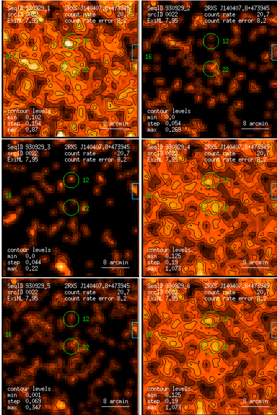
Figure 22: RASS 930929: detection 0022: band rate images, Gaussian filter: (1) PSPC channels 11 – 41, (2) 52 – 90, (3) 91 – 201, (4) 11 – 235, (5) 52 – 201, (6) 11 – 201. Broad band rates in counts/ks. Band rate contour levels in counts/ks/arcmin 2 .
