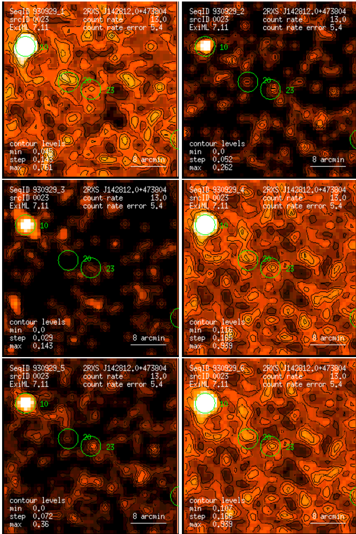
Figure 23: RASS 930929: detection 0023: band rate images, Gaussian filter: (1) PSPC channels 11 – 41, (2) 52 – 90, (3) 91 – 201, (4) 11 – 235, (5) 52 – 201, (6) 11 – 201. Broad band rates in counts/ks. Band rate contour levels in counts/ks/arcmin 2 .
