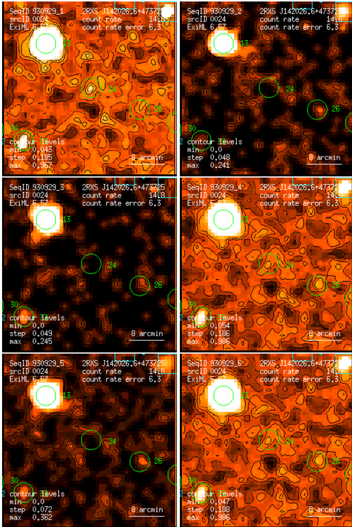
Figure 24: RASS 930929: detection 0024: band rate images, Gaussian filter: (1) PSPC channels 11 – 41, (2) 52 – 90, (3) 91 – 201, (4) 11 – 235, (5) 52 – 201, (6) 11 – 201. Broad band rates in counts/ks. Band rate contour levels in counts/ks/arcmin 2 .
