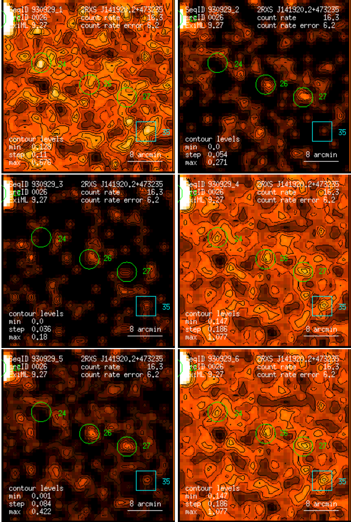
Figure 26: RASS 930929: detection 0026: band rate images, Gaussian filter: (1) PSPC channels 11 – 41, (2) 52 – 90, (3) 91 – 201, (4) 11 – 235, (5) 52 – 201, (6) 11 – 201. Broad band rates in counts/ks. Band rate contour levels in counts/ks/arcmin 2 .
