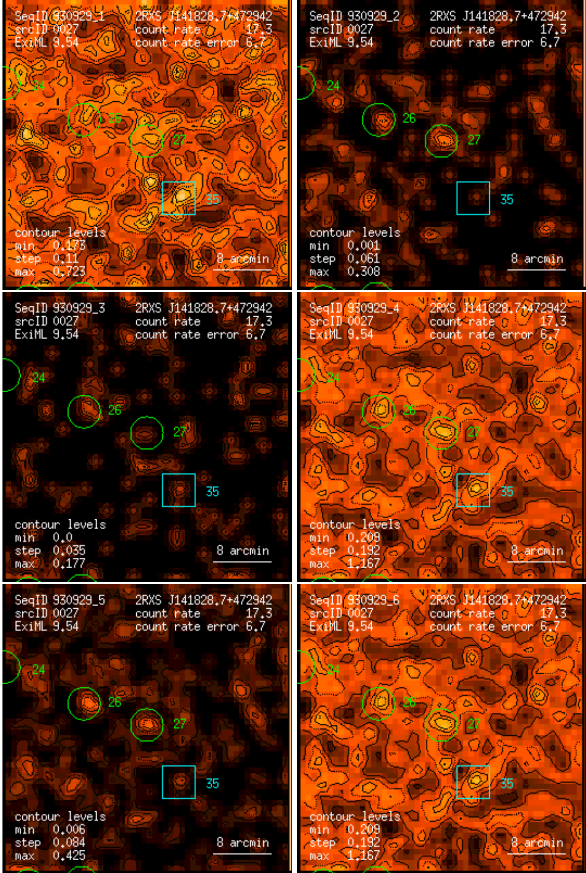
Figure 27: RASS 930929: detection 0027: band rate images, Gaussian filter: (1) PSPC channels 11 – 41, (2) 52 – 90, (3) 91 – 201, (4) 11 – 235, (5) 52 – 201, (6) 11 – 201. Broad band rates in counts/ks. Band rate contour levels in counts/ks/arcmin 2 .
