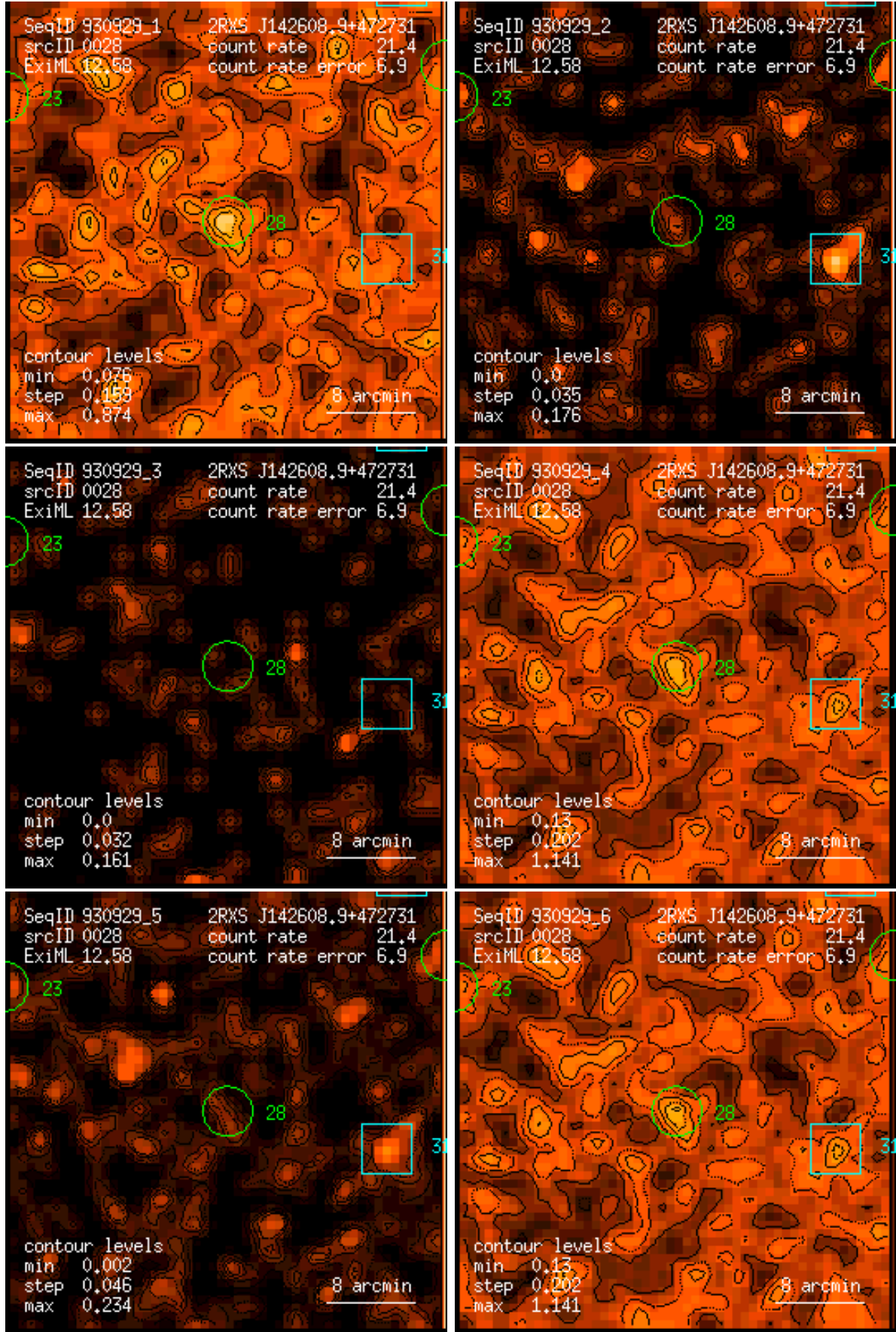
Figure 28: RASS 930929: detection 0028: band rate images, Gaussian filter: (1) PSPC channels 11 – 41, (2) 52 – 90, (3) 91 – 201, (4) 11 – 235, (5) 52 – 201, (6) 11 – 201. Broad band rates in counts/ks. Band rate contour levels in counts/ks/arcmin 2 .
