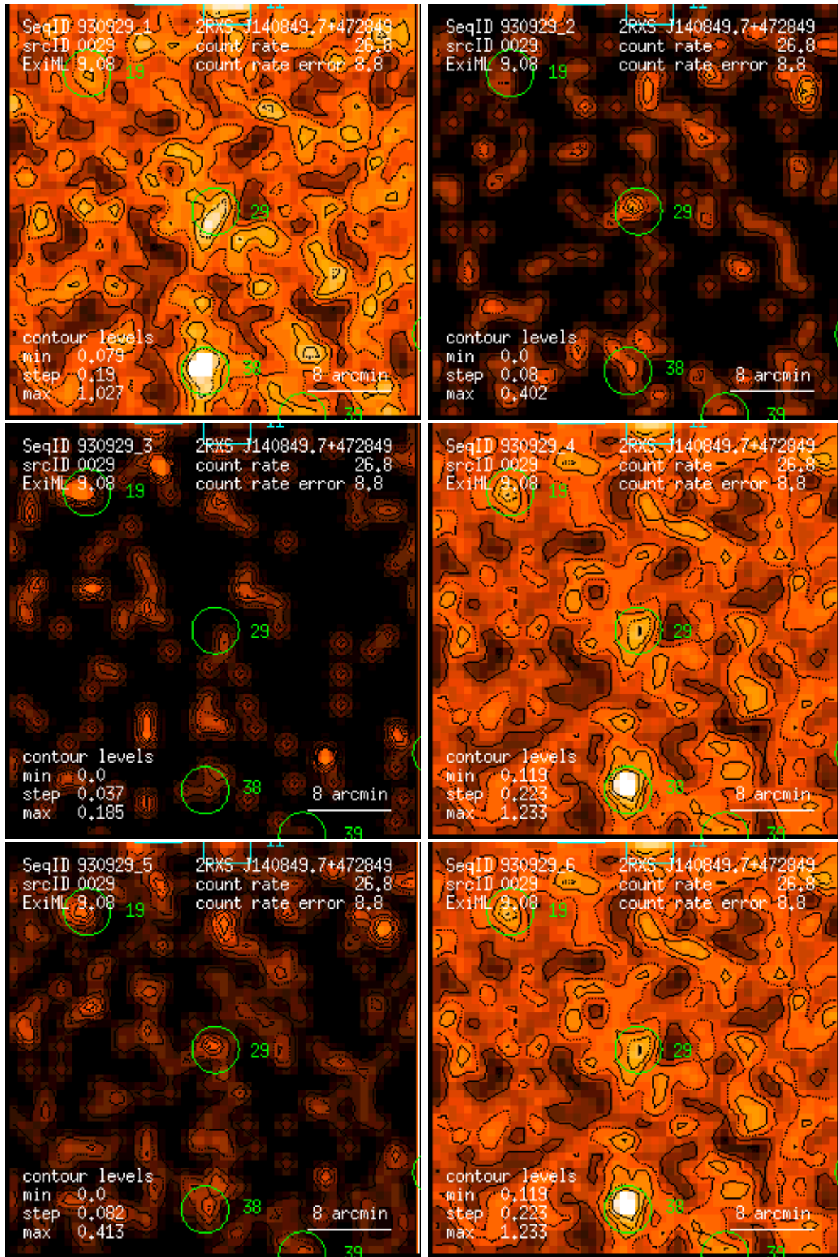
Figure 29: RASS 930929: detection 0029: band rate images, Gaussian filter: (1) PSPC channels 11 – 41, (2) 52 – 90, (3) 91 – 201, (4) 11 – 235, (5) 52 – 201, (6) 11 – 201. Broad band rates in counts/ks. Band rate contour levels in counts/ks/arcmin 2 .
