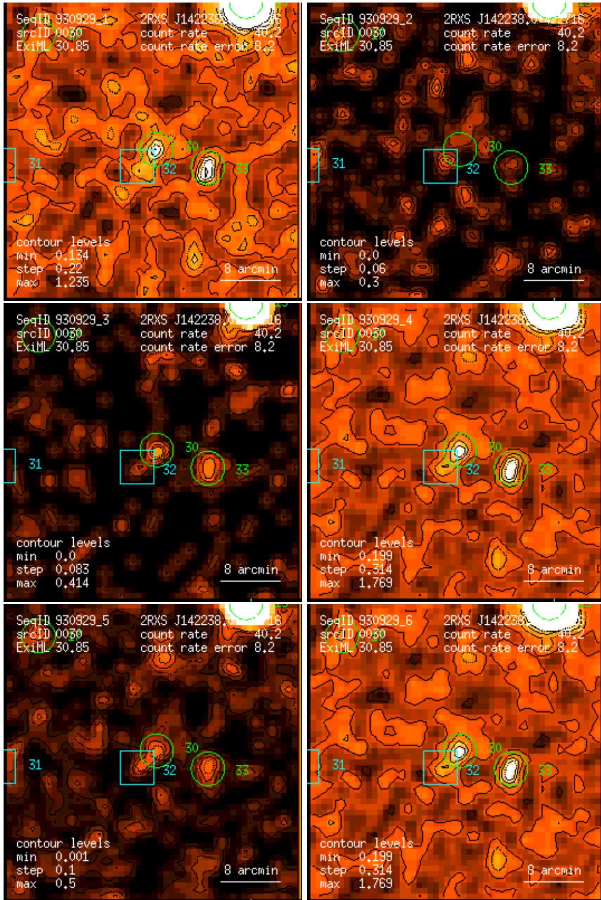
Figure 30: RASS 930929: detection 0030: band rate images, Gaussian filter: (1) PSPC channels 11 – 41, (2) 52 – 90, (3) 91 – 201, (4) 11 – 235, (5) 52 – 201, (6) 11 – 201. Broad band rates in counts/ks. Band rate contour levels in counts/ks/arcmin 2 .
