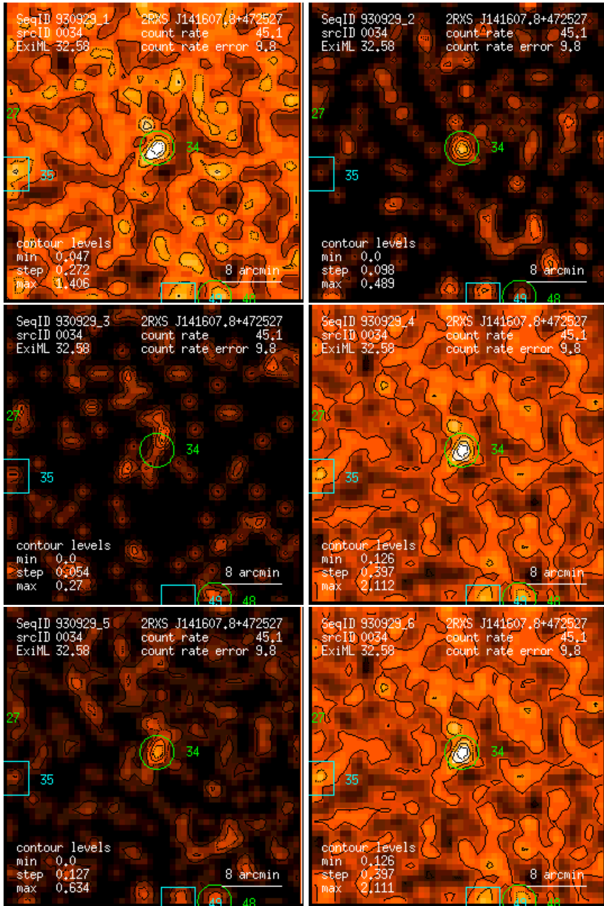
Figure 34: RASS 930929: detection 0034: band rate images, Gaussian filter: (1) PSPC channels 11 – 41, (2) 52 – 90, (3) 91 – 201, (4) 11 – 235, (5) 52 – 201, (6) 11 – 201. Broad band rates in counts/ks. Band rate contour levels in counts/ks/arcmin 2 .
