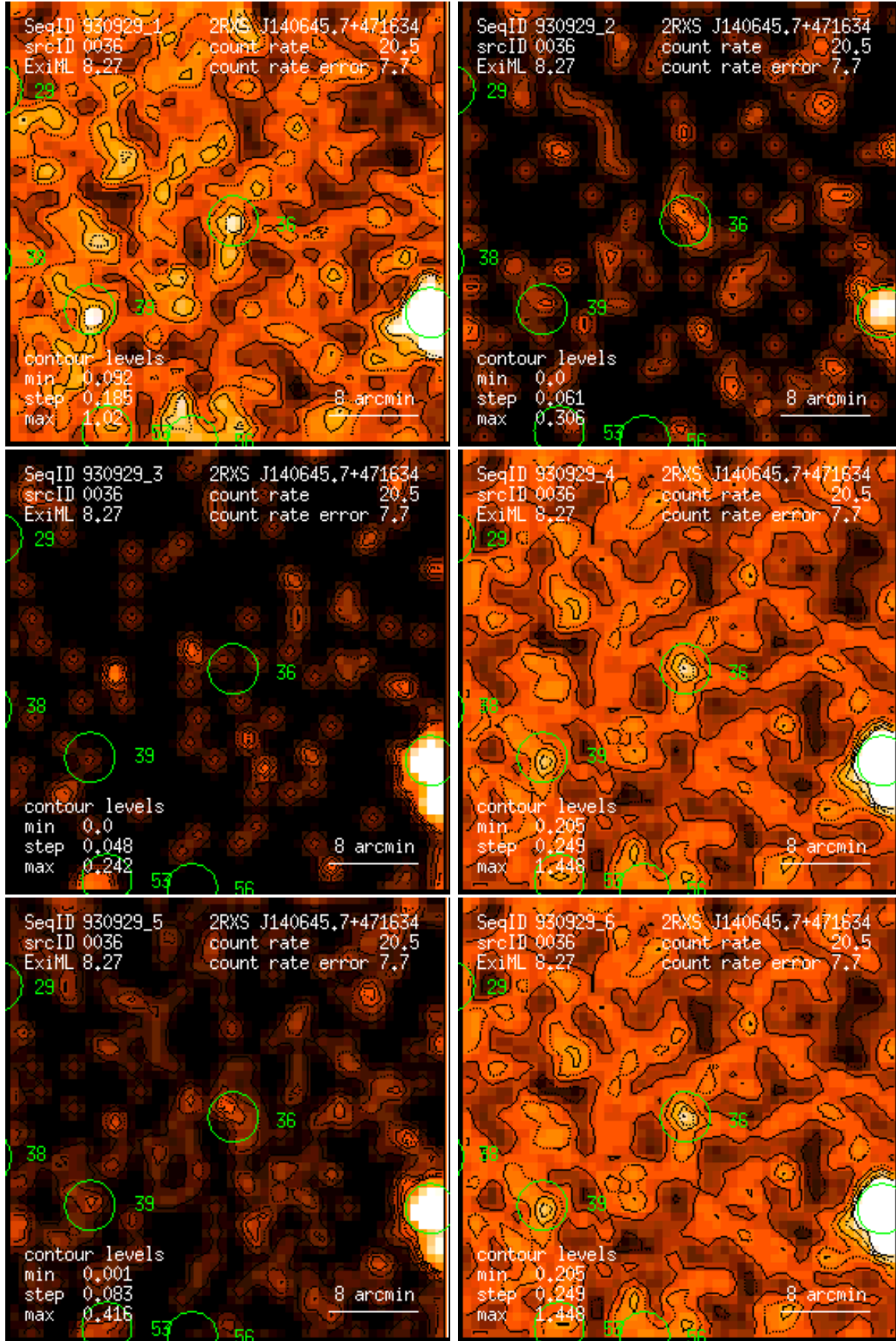
Figure 36: RASS 930929: detection 0036: band rate images, Gaussian filter: (1) PSPC channels 11 – 41, (2) 52 – 90, (3) 91 – 201, (4) 11 – 235, (5) 52 – 201, (6) 11 – 201. Broad band rates in counts/ks. Band rate contour levels in counts/ks/arcmin 2 .
