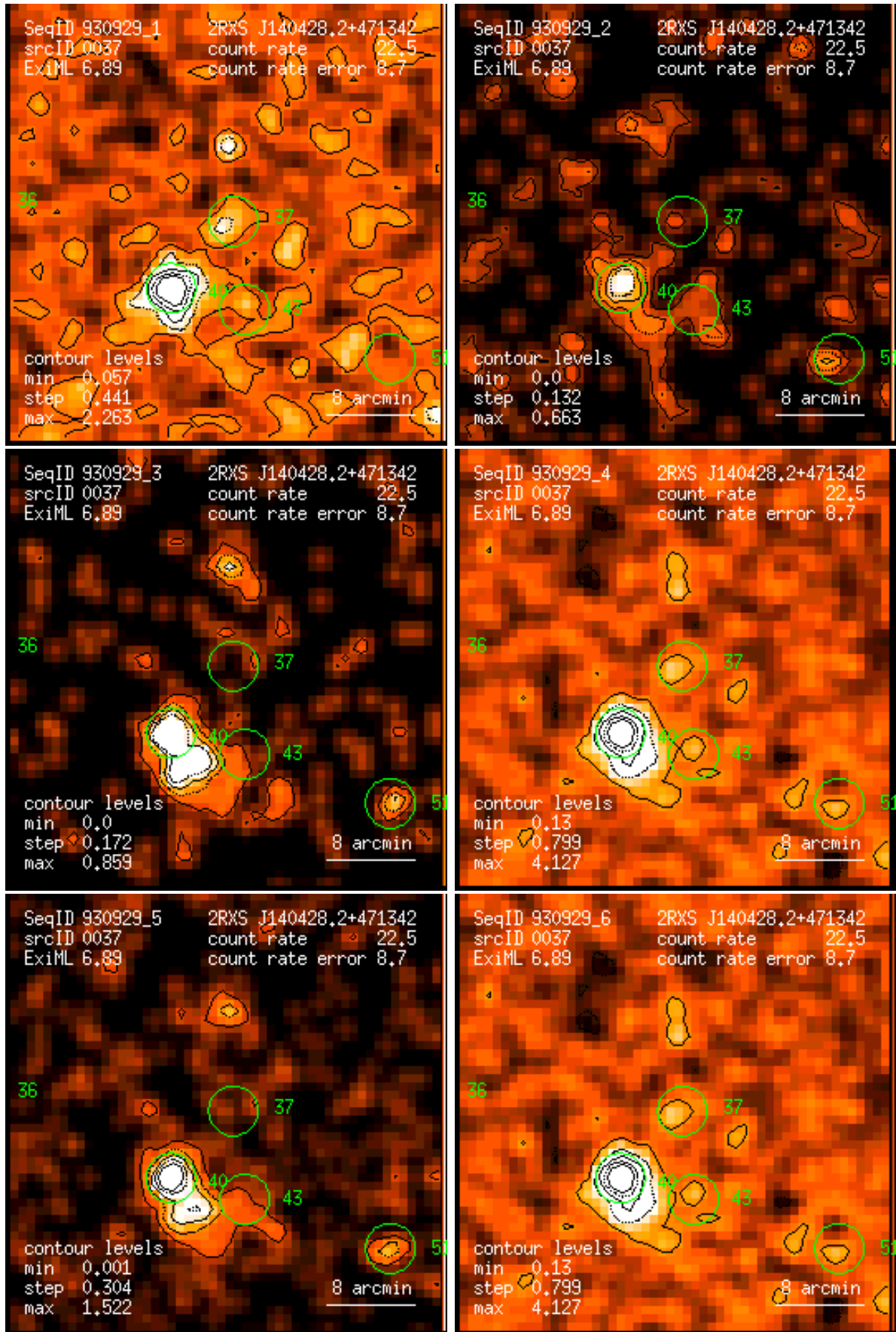
Figure 37: RASS 930929: detection 0037: band rate images, Gaussian filter: (1) PSPC channels 11 – 41, (2) 52 – 90, (3) 91 – 201, (4) 11 – 235, (5) 52 – 201, (6) 11 – 201. Broad band rates in counts/ks. Band rate contour levels in counts/ks/arcmin 2 .
