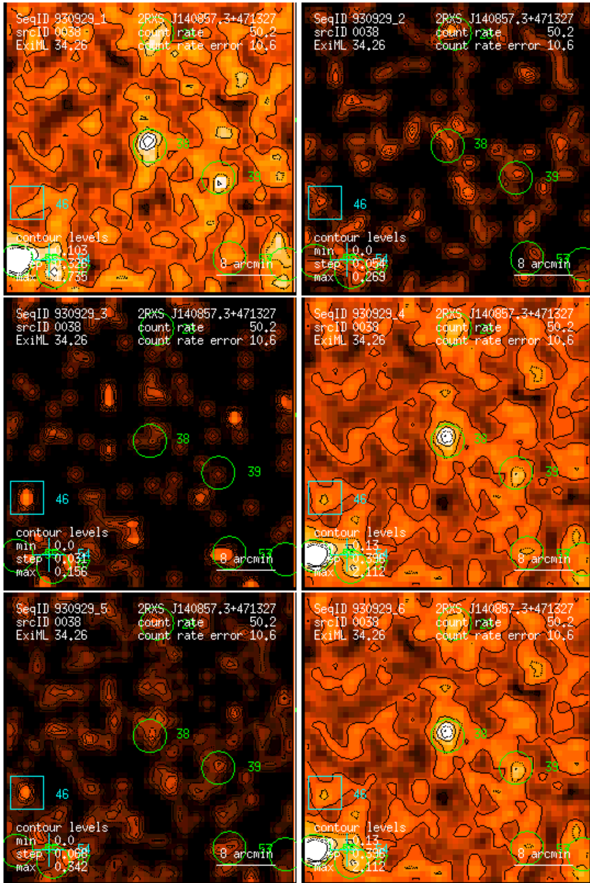
Figure 38: RASS 930929: detection 0038: band rate images, Gaussian filter: (1) PSPC channels 11 – 41, (2) 52 – 90, (3) 91 – 201, (4) 11 – 235, (5) 52 – 201, (6) 11 – 201. Broad band rates in counts/ks. Band rate contour levels in counts/ks/arcmin 2 .
