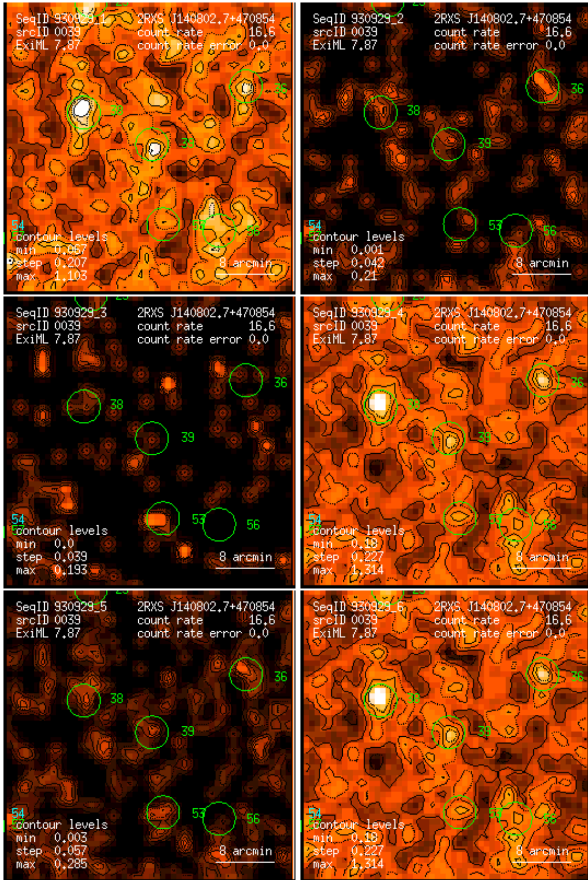
Figure 39: RASS 930929: detection 0039: band rate images, Gaussian filter: (1) PSPC channels 11 – 41, (2) 52 – 90, (3) 91 – 201, (4) 11 – 235, (5) 52 – 201, (6) 11 – 201. Broad band rates in counts/ks. Band rate contour levels in counts/ks/arcmin 2 .
