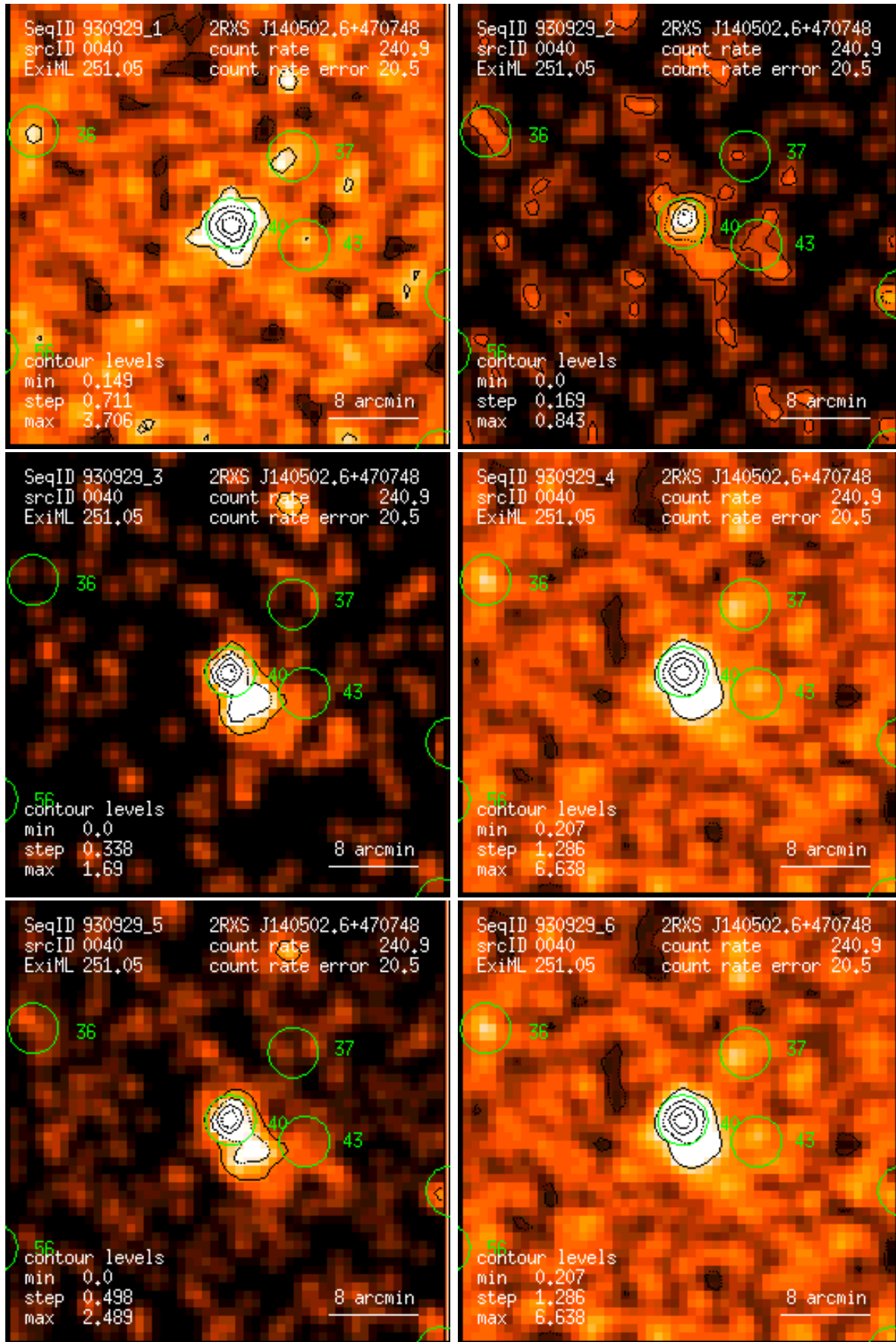
Figure 40: RASS 930929: detection 0040: band rate images, Gaussian filter: (1) PSPC channels 11 – 41, (2) 52 – 90, (3) 91 – 201, (4) 11 – 235, (5) 52 – 201, (6) 11 – 201. Broad band rates in counts/ks. Band rate contour levels in counts/ks/arcmin 2 .
