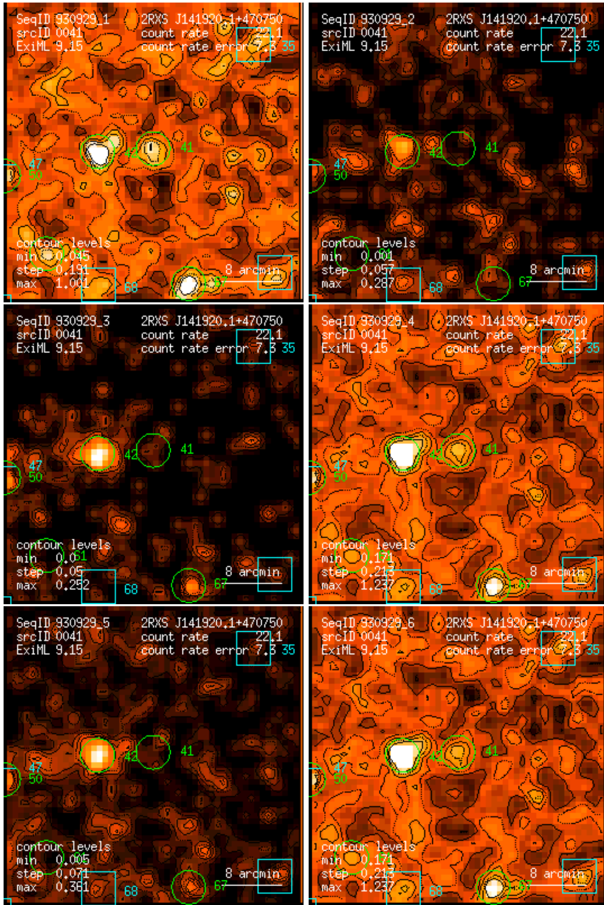
Figure 41: RASS 930929: detection 0041: band rate images, Gaussian filter: (1) PSPC channels 11 – 41, (2) 52 – 90, (3) 91 – 201, (4) 11 – 235, (5) 52 – 201, (6) 11 – 201. Broad band rates in counts/ks. Band rate contour levels in counts/ks/arcmin 2 .
