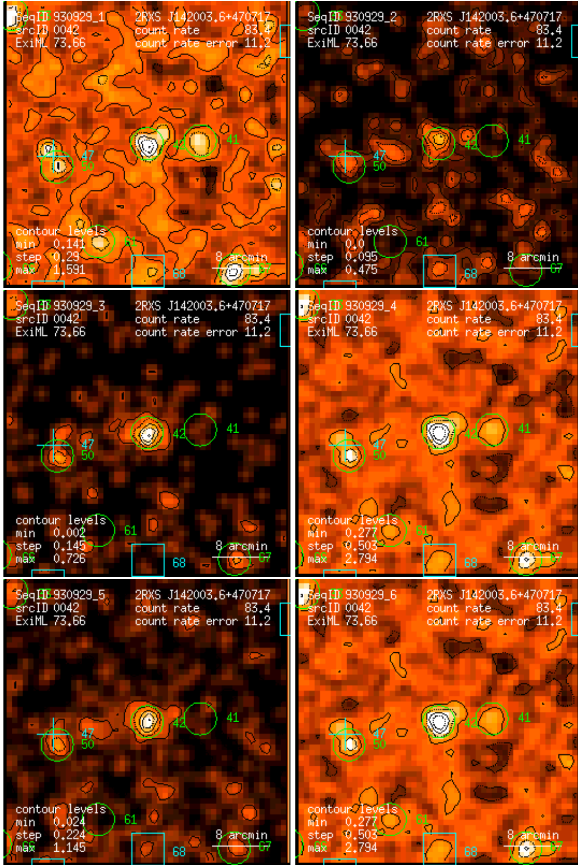
Figure 42: RASS 930929: detection 0042: band rate images, Gaussian filter: (1) PSPC channels 11 – 41, (2) 52 – 90, (3) 91 – 201, (4) 11 – 235, (5) 52 – 201, (6) 11 – 201. Broad band rates in counts/ks. Band rate contour levels in counts/ks/arcmin 2 .
