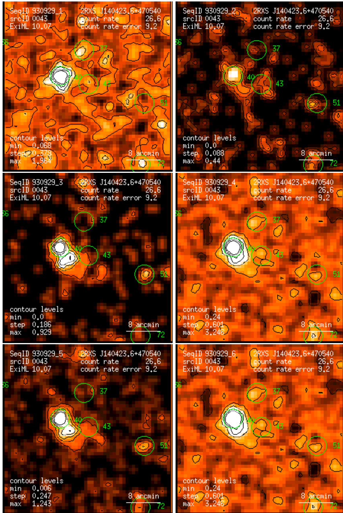
Figure 43: RASS 930929: detection 0043: band rate images, Gaussian filter: (1) PSPC channels 11 – 41, (2) 52 – 90, (3) 91 – 201, (4) 11 – 235, (5) 52 – 201, (6) 11 – 201. Broad band rates in counts/ks. Band rate contour levels in counts/ks/arcmin 2 .
