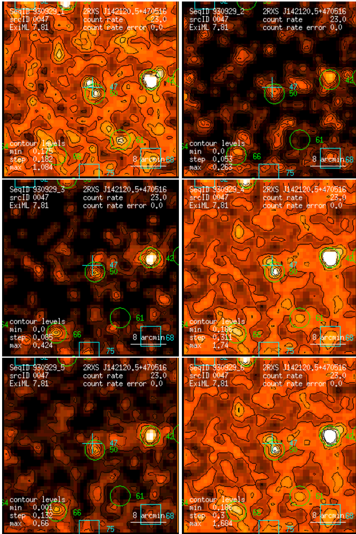
Figure 47: RASS 930929: detection 0047: band rate images, Gaussian filter: (1) PSPC channels 11 – 41, (2) 52 – 90, (3) 91 – 201, (4) 11 – 235, (5) 52 – 201, (6) 11 – 201. Broad band rates in counts/ks. Band rate contour levels in counts/ks/arcmin 2 .
