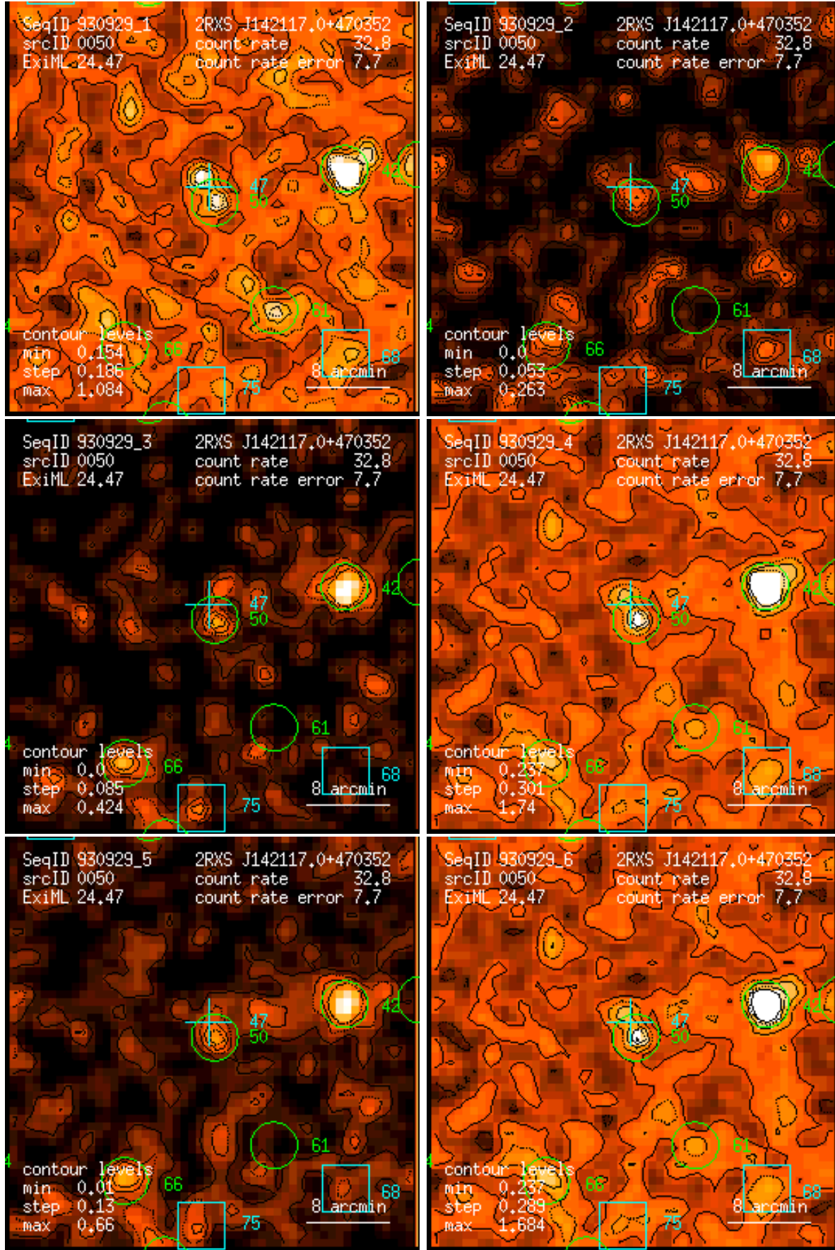
Figure 50: RASS 930929: detection 0050: band rate images, Gaussian filter: (1) PSPC channels 11 – 41, (2) 52 – 90, (3) 91 – 201, (4) 11 – 235, (5) 52 – 201, (6) 11 – 201. Broad band rates in counts/ks. Band rate contour levels in counts/ks/arcmin 2 .
