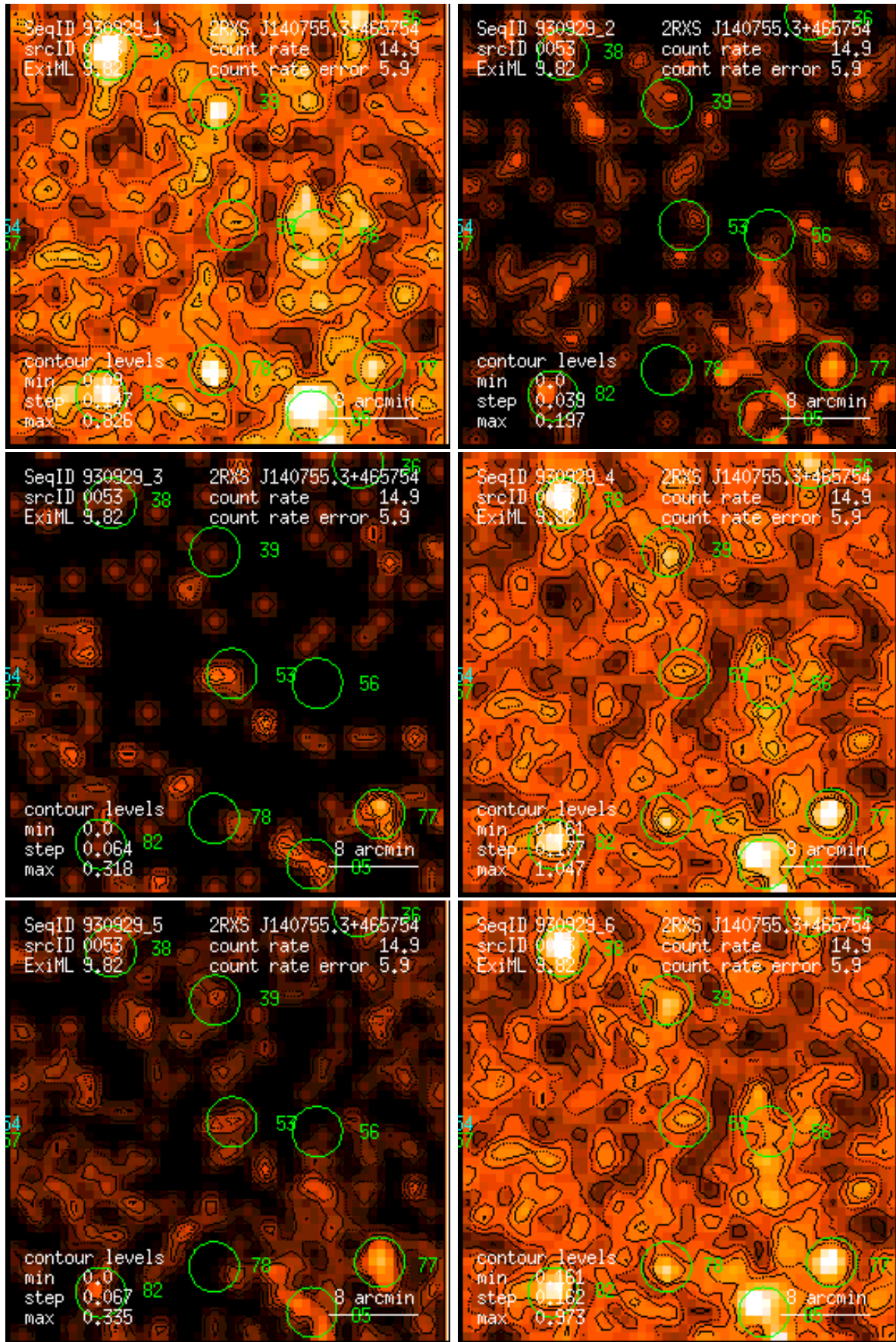
Figure 53: RASS 930929: detection 0053: band rate images, Gaussian filter: (1) PSPC channels 11 – 41, (2) 52 – 90, (3) 91 – 201, (4) 11 – 235, (5) 52 – 201, (6) 11 – 201. Broad band rates in counts/ks. Band rate contour levels in counts/ks/arcmin 2 .
