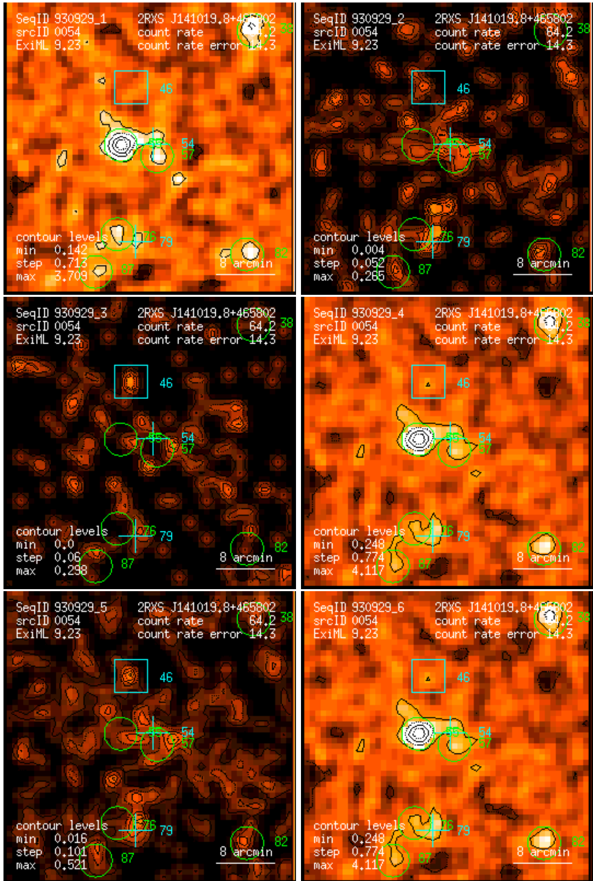
Figure 54: RASS 930929: detection 0054: band rate images, Gaussian filter: (1) PSPC channels 11 – 41, (2) 52 – 90, (3) 91 – 201, (4) 11 – 235, (5) 52 – 201, (6) 11 – 201. Broad band rates in counts/ks. Band rate contour levels in counts/ks/arcmin 2 .
