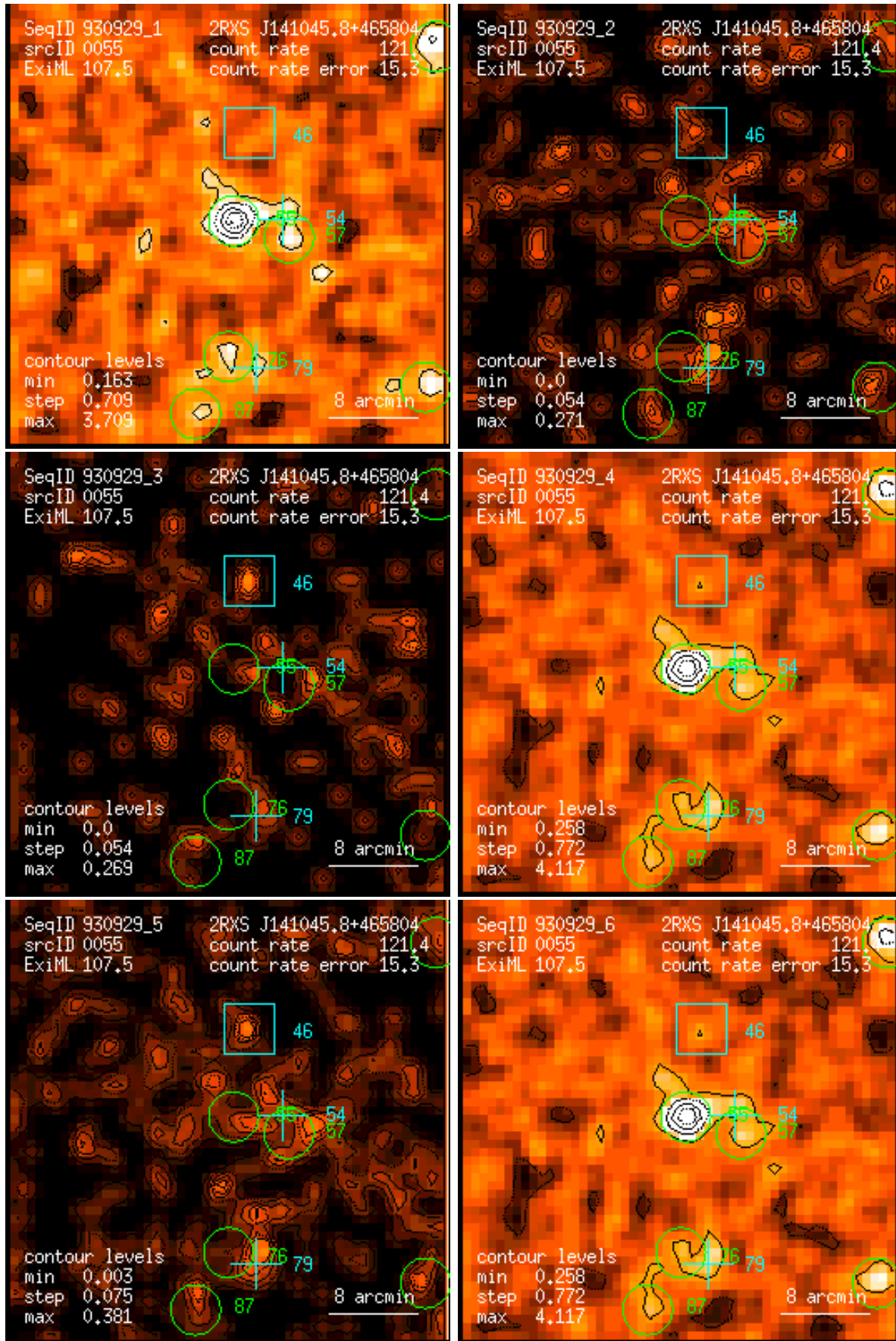
Figure 55: RASS 930929: detection 0055: band rate images, Gaussian filter: (1) PSPC channels 11 – 41, (2) 52 – 90, (3) 91 – 201, (4) 11 – 235, (5) 52 – 201, (6) 11 – 201. Broad band rates in counts/ks. Band rate contour levels in counts/ks/arcmin 2 .
