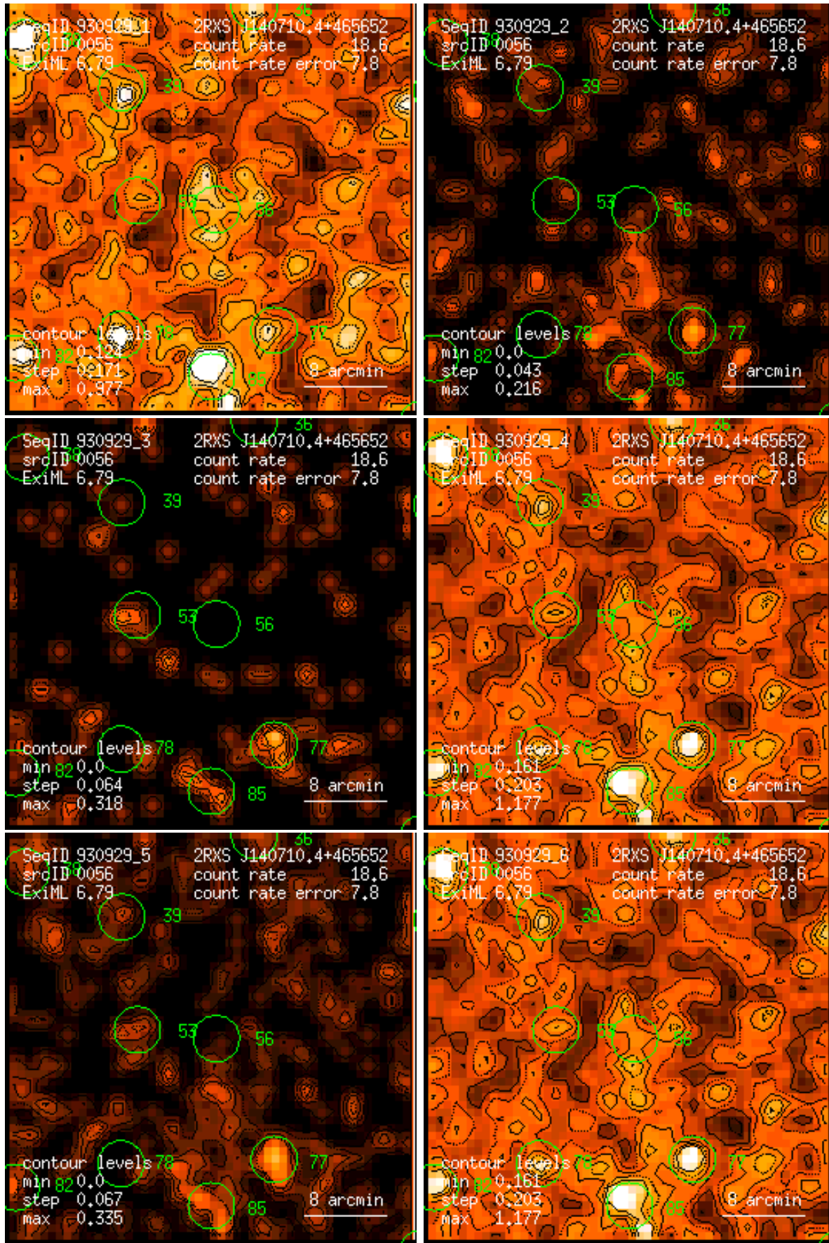
Figure 56: RASS 930929: detection 0056: band rate images, Gaussian filter: (1) PSPC channels 11 – 41, (2) 52 – 90, (3) 91 – 201, (4) 11 – 235, (5) 52 – 201, (6) 11 – 201. Broad band rates in counts/ks. Band rate contour levels in counts/ks/arcmin 2 .
