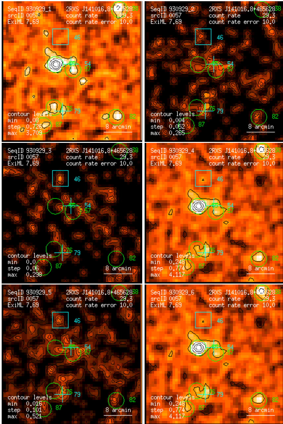
Figure 57: RASS 930929: detection 0057: band rate images, Gaussian filter: (1) PSPC channels 11 – 41, (2) 52 – 90, (3) 91 – 201, (4) 11 – 235, (5) 52 – 201, (6) 11 – 201. Broad band rates in counts/ks. Band rate contour levels in counts/ks/arcmin 2 .
