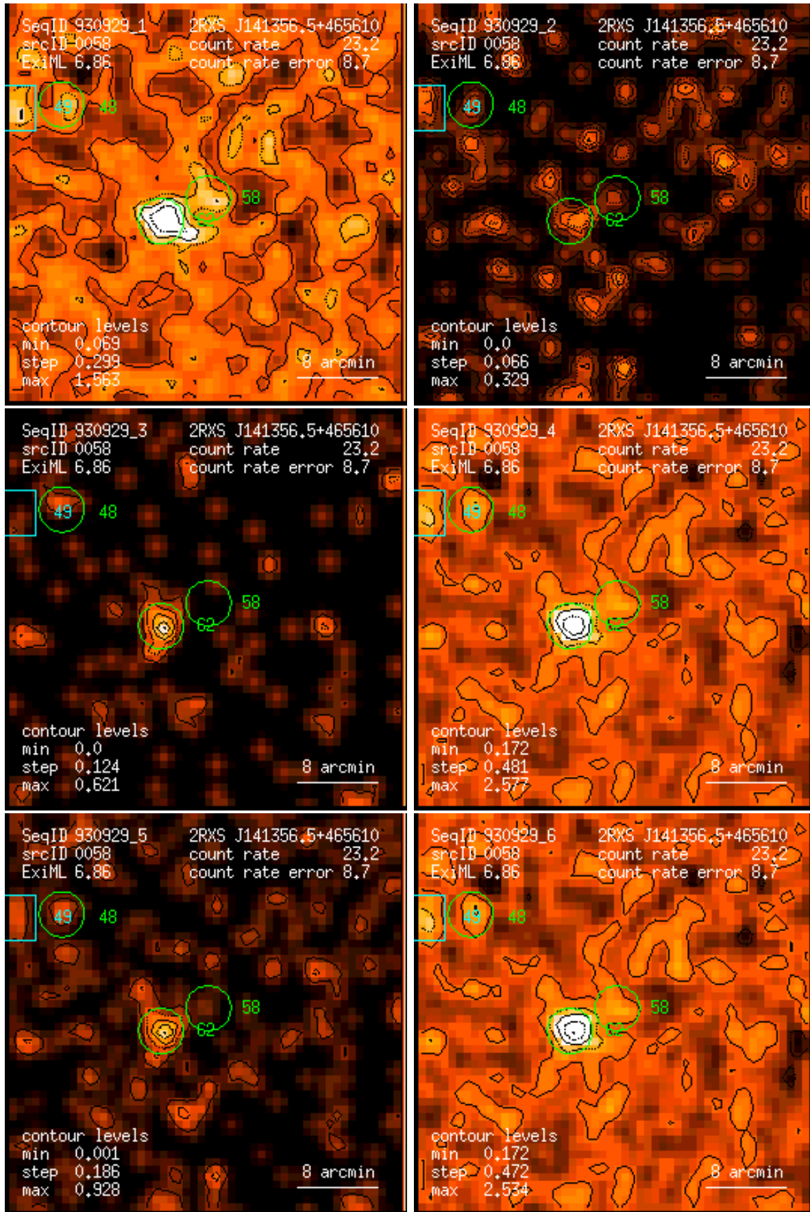
Figure 58: RASS 930929: detection 0058: band rate images, Gaussian filter: (1) PSPC channels 11 – 41, (2) 52 – 90, (3) 91 – 201, (4) 11 – 235, (5) 52 – 201, (6) 11 – 201. Broad band rates in counts/ks. Band rate contour levels in counts/ks/arcmin 2 .
