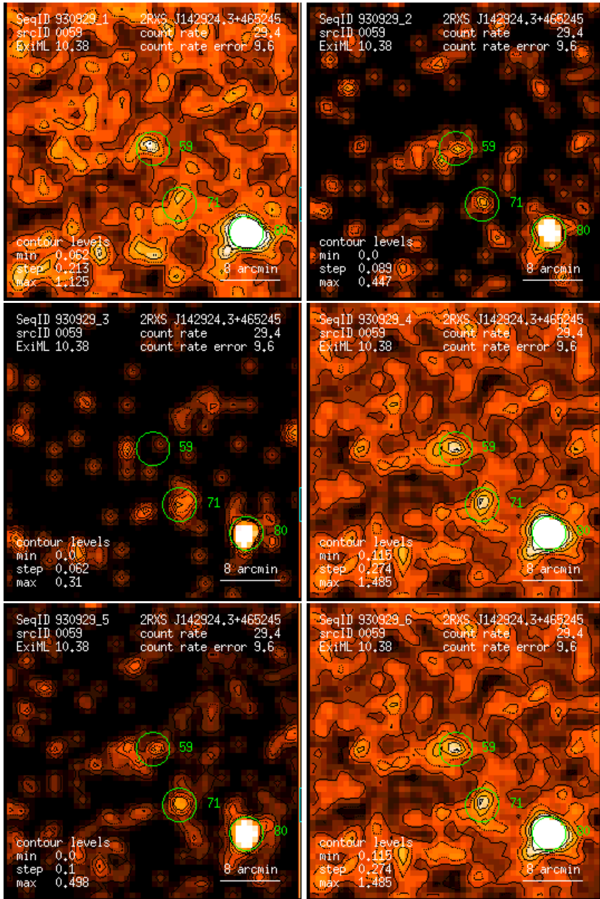
Figure 59: RASS 930929: detection 0059: band rate images, Gaussian filter: (1) PSPC channels 11 – 41, (2) 52 – 90, (3) 91 – 201, (4) 11 – 235, (5) 52 – 201, (6) 11 – 201. Broad band rates in counts/ks. Band rate contour levels in counts/ks/arcmin 2 .
