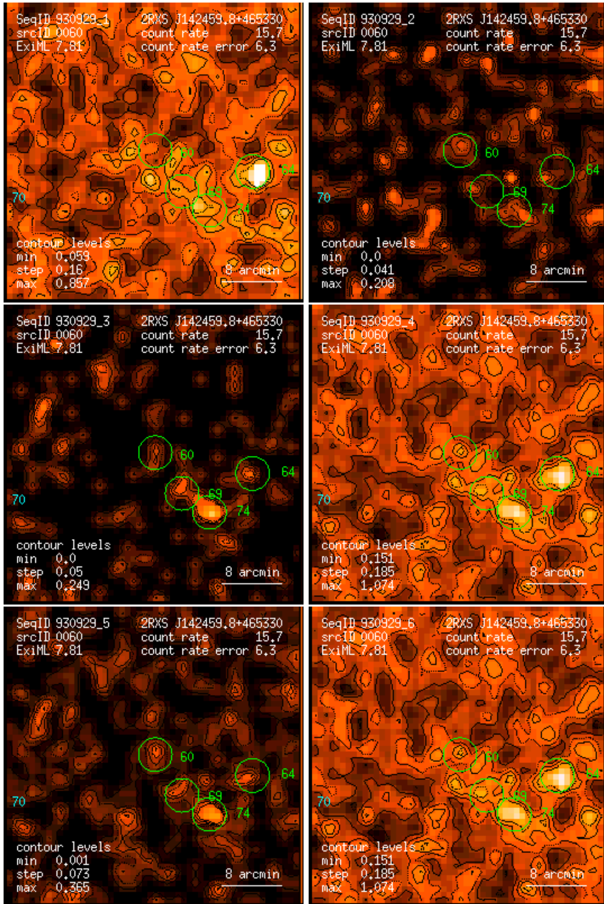
Figure 60: RASS 930929: detection 0060: band rate images, Gaussian filter: (1) PSPC channels 11 – 41, (2) 52 – 90, (3) 91 – 201, (4) 11 – 235, (5) 52 – 201, (6) 11 – 201. Broad band rates in counts/ks. Band rate contour levels in counts/ks/arcmin 2 .
