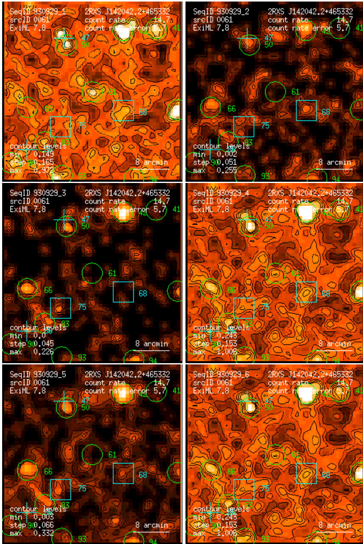
Figure 61: RASS 930929: detection 0061: band rate images, Gaussian filter: (1) PSPC channels 11 – 41, (2) 52 – 90, (3) 91 – 201, (4) 11 – 235, (5) 52 – 201, (6) 11 – 201. Broad band rates in counts/ks. Band rate contour levels in counts/ks/arcmin 2 .
