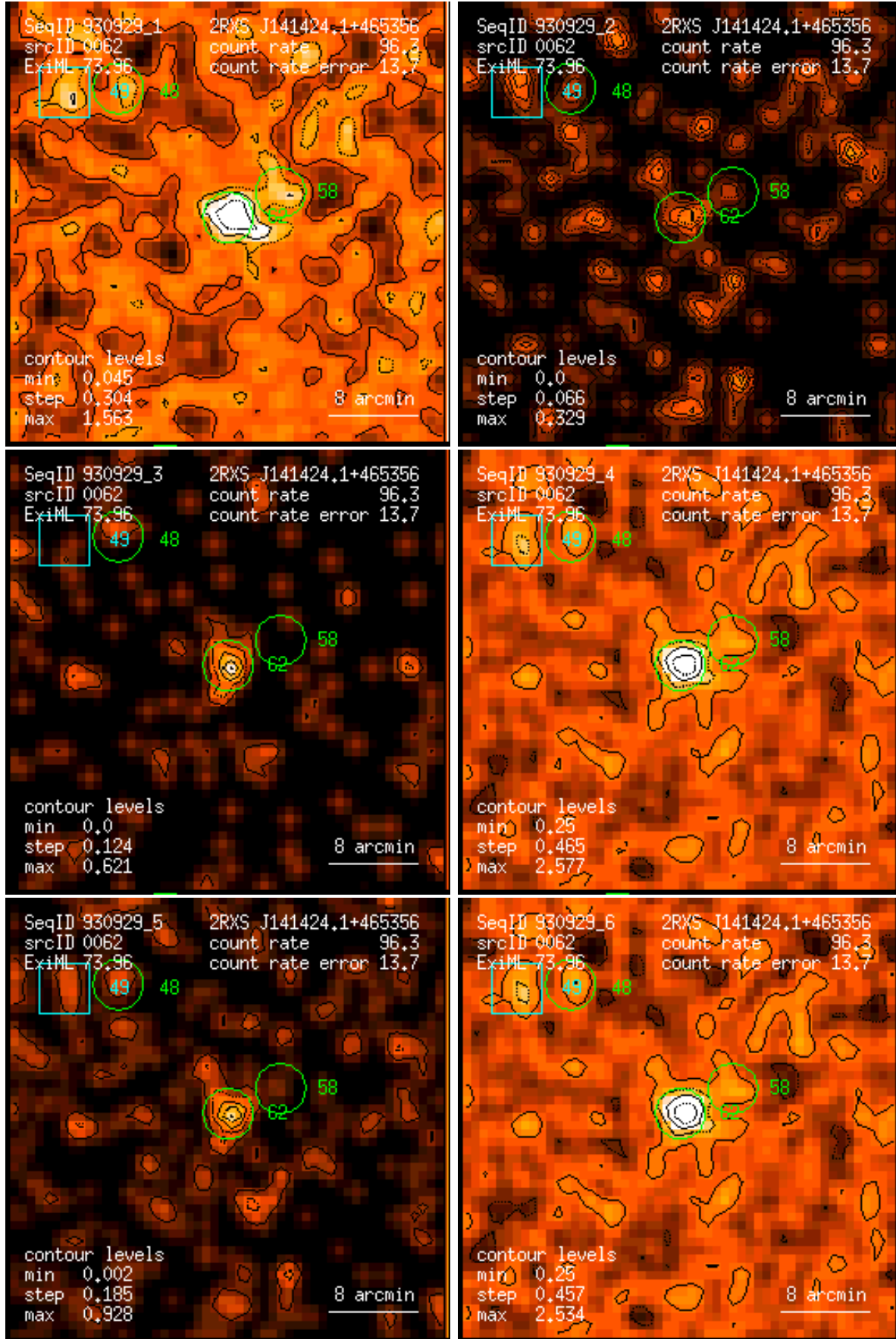
Figure 62: RASS 930929: detection 0062: band rate images, Gaussian filter: (1) PSPC channels 11 – 41, (2) 52 – 90, (3) 91 – 201, (4) 11 – 235, (5) 52 – 201, (6) 11 – 201. Broad band rates in counts/ks. Band rate contour levels in counts/ks/arcmin 2 .
