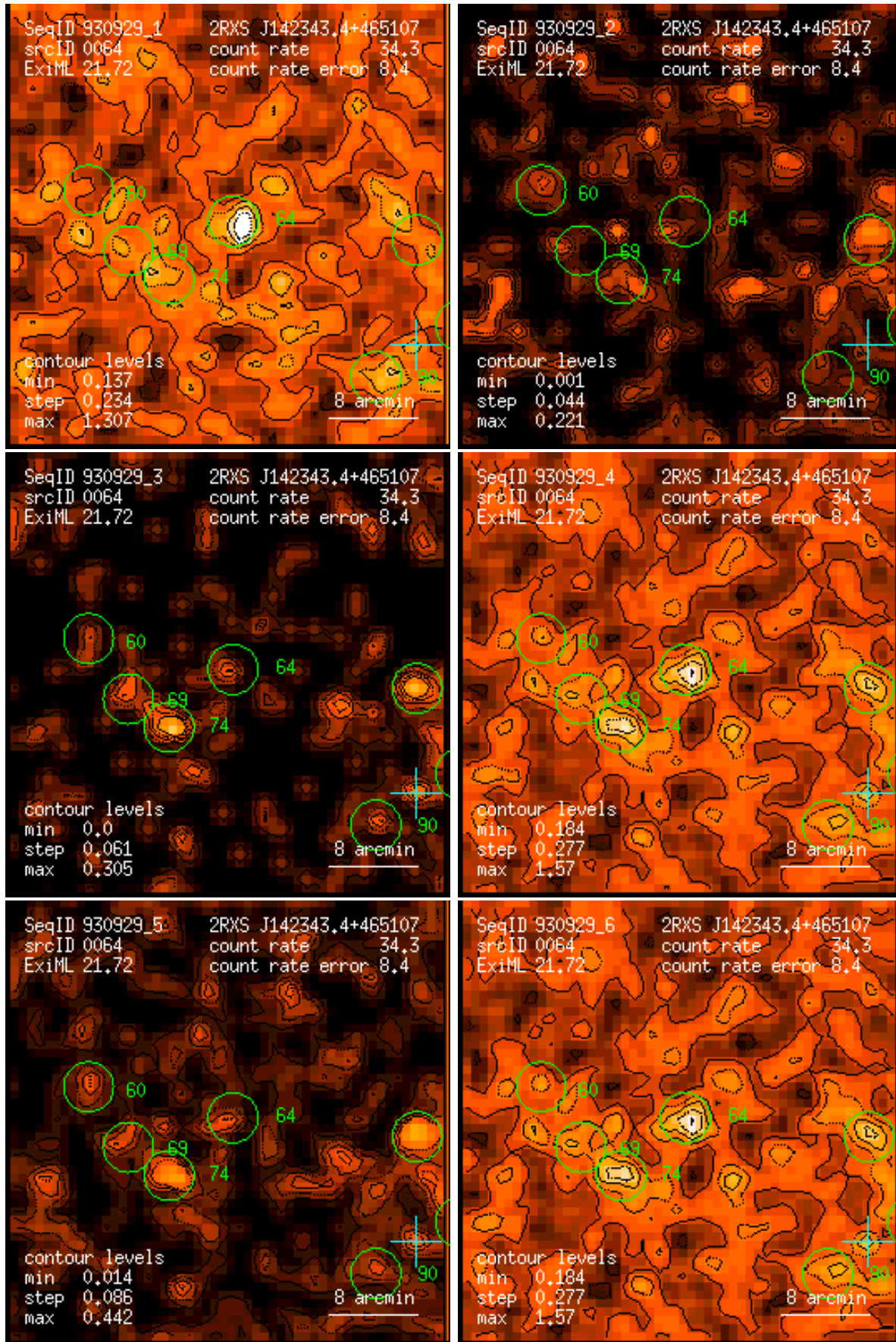
Figure 64: RASS 930929: detection 0064: band rate images, Gaussian filter: (1) PSPC channels 11 – 41, (2) 52 – 90, (3) 91 – 201, (4) 11 – 235, (5) 52 – 201, (6) 11 – 201. Broad band rates in counts/ks. Band rate contour levels in counts/ks/arcmin 2 .
