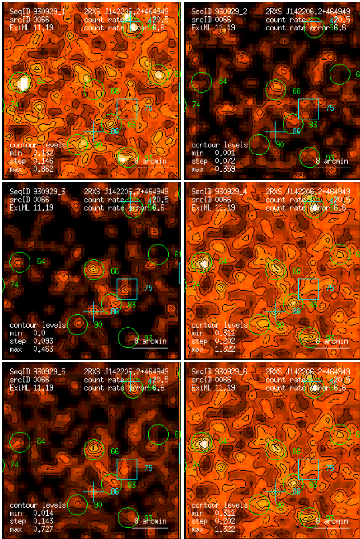
Figure 66: RASS 930929: detection 0066: band rate images, Gaussian filter: (1) PSPC channels 11 – 41, (2) 52 – 90, (3) 91 – 201, (4) 11 – 235, (5) 52 – 201, (6) 11 – 201. Broad band rates in counts/ks. Band rate contour levels in counts/ks/arcmin 2 .
