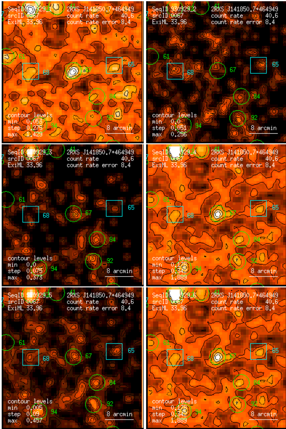
Figure 67: RASS 930929: detection 0067: band rate images, Gaussian filter: (1) PSPC channels 11 – 41, (2) 52 – 90, (3) 91 – 201, (4) 11 – 235, (5) 52 – 201, (6) 11 – 201. Broad band rates in counts/ks. Band rate contour levels in counts/ks/arcmin 2 .
