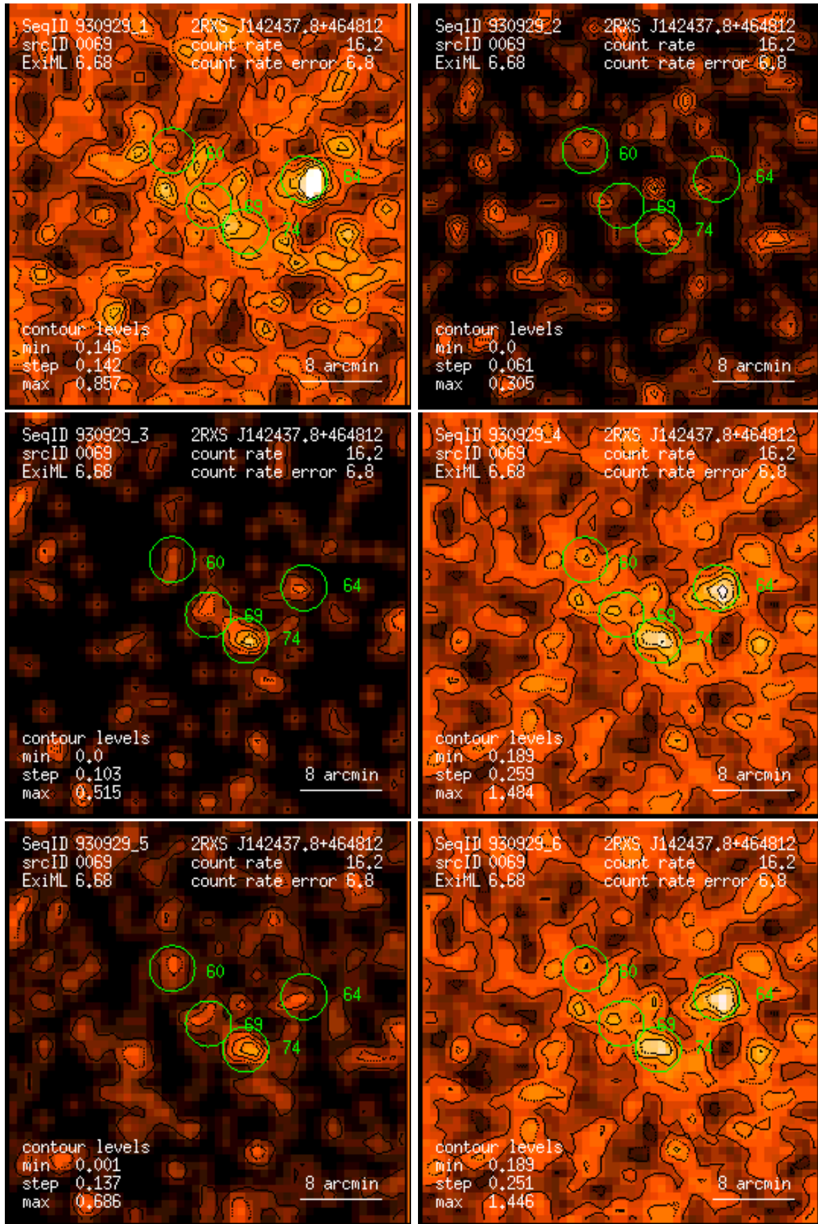
Figure 69: RASS 930929: detection 0069: band rate images, Gaussian filter: (1) PSPC channels 11 – 41, (2) 52 – 90, (3) 91 – 201, (4) 11 – 235, (5) 52 – 201, (6) 11 – 201. Broad band rates in counts/ks. Band rate contour levels in counts/ks/arcmin 2 .
